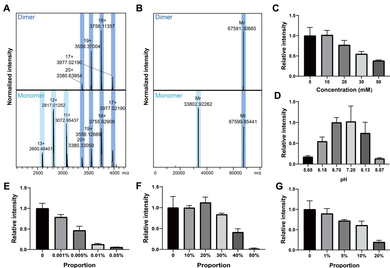
Fig. 1. Spray condition optimization for 3CLpro. Raw MS spectra (A) and deconvoluted spectra (B) of 3CLpro mainly in dimer (dark blue) or monomer (light blue) states. (C) The intensity of 3CLpro in NH 4 Ac at different concentrations. (D) The intensity of 3CLpro in 10 mM NH 4 Ac at different pH values. The influence of different proportions of DMSO (E), MeOH (F), or ACN (G) on the spray system. Experiments were repeated at least three times. Bars represent mean \pm SD.
