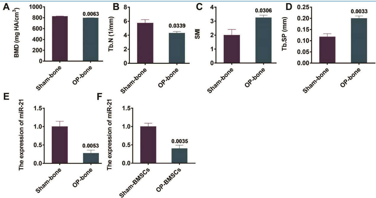
Figure 1. Expression of miR-21 in OP mice. (A-D) Detection of bone-related indexes by microCT, SMI = structure model index; (E) qRT-PCR detection of the expression of miR-21 in bone tissue of OP mice; (F) qRT-PCR detection of the expression of miR-21 in mouse BMSCs in OP group.
