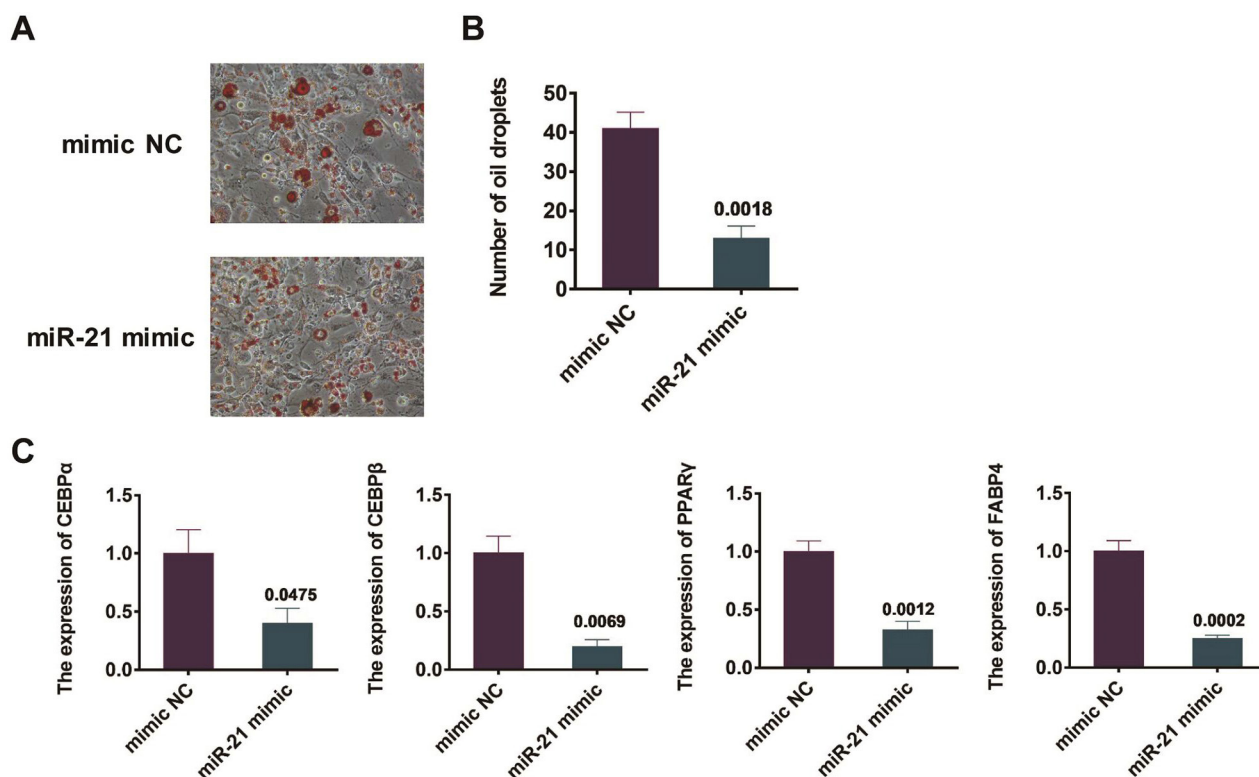
Figure 4. Effect of overexpression of miR-21 on adipogenic differentiation of mouse BMSCs. (A) Detection of the formation of lipid droplets in BMSCs by oil red O staining; (B) Quantitative results of oil red O staining; (C) Detection of the expression levels of adipogenesis related genes CEBP \alpha , CEBP \beta , FABP4 and PPAR \gamma in mouse BMSCs by qRT-PCR.
