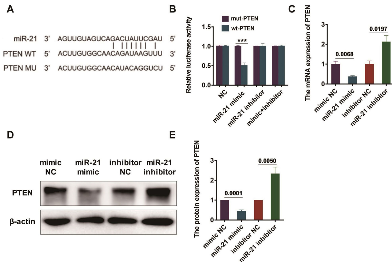
Figure 5. miR-21 negatively regulates PTEN expression. (A) The binding site of miR-21 and PTEN; (B) Luciferase reporter assay was used to detect the regulatory association between miR-21 and PTEN; (C) Detection of PTEN mRNA expression by qRT-PCR; (D) Detection of the protein expression of PTEN was observed by western blot; (E) Statistical results of western blot.
