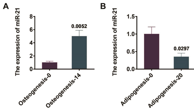
Figure 2. miR-21 expression changes before and after differentiation in BMSCs of mice. (A) qRT-PCR detection of the expression of miR-21 before and after osteogenesis of mouse BMSCs; (B) qRT-PCR detection of the expression of miR-21 before and after adipogenesis of mouse BMSCs.
