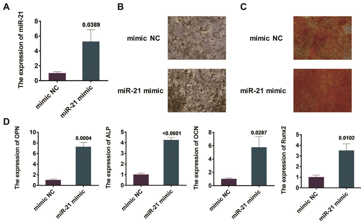
Figure 3. Effects of overexpression of miR-21 on osteogenic differentiation of mouse BMSCs. (A) Observation of miR-21 expression in mouse BMSCs by qRT-PCR; (B) Detection of calcium nodule formation in BMSCs by alkaline phosphatase staining; (C) Manifestation of calcium nodule emergence in BMSCs by Alizarin red staining; (D) Detection of the expression degrees of osteogenesis-related genes Runx2, ALP, OCN and OPN in mouse BMSCs by qRT-PCR.
