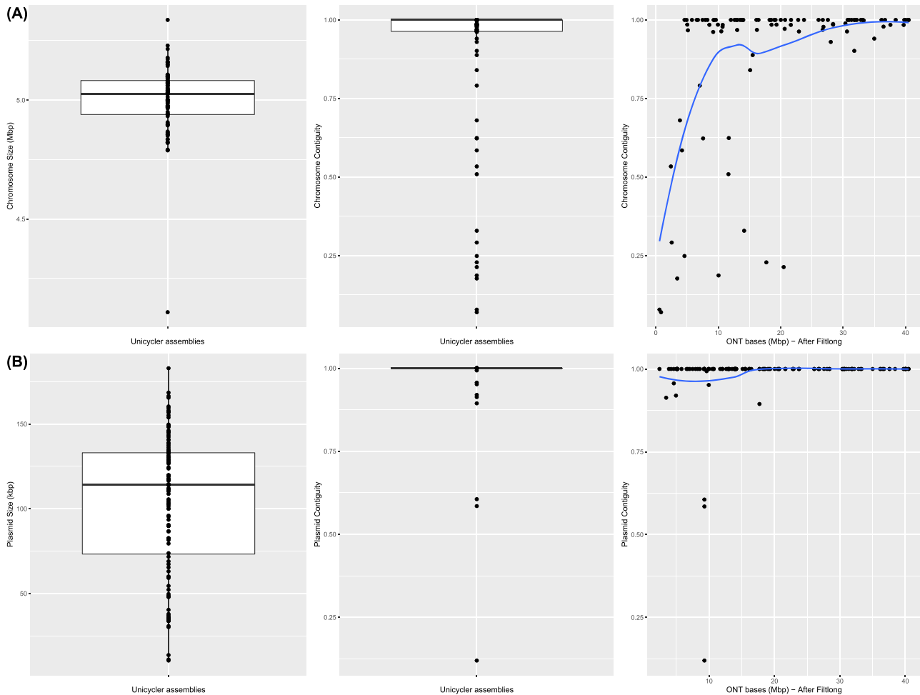
Figure 3. Unicycler statistics for the 96 isolates included in the ONT sequencing. Boxplots showing the component size (left) and contiguity values (middle) together with an evaluation of the correlation between the number of ONT bases generated and the contiguity values achieved (right). (A) Statistics for the chromosome component (largest component); the largest contig was confirmed as chromosome-derived with mlplasmids . (B) Statistics for medium and large plasmid components (size > 10 kb); the largest contig was confirmed as plasmid-derived with mlplasmids .
