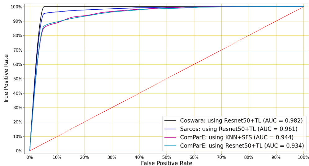
Fig. 5. COVID-19 cough classification: A Resnet50 classifier with transfer learning achieved the highest AUC in classifying COVID-19 coughs for the Coswara and Sarcos datasets (0.982 and 0.961 respectively). For the ComParE dataset, AUCs of 0.944 and 0.934 were achieved by a KNN classifier using 12 features identified by SFS and by a Resnet50 classifier trained by transfer learning respectively.
