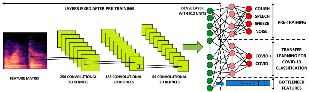
Fig. 4. CNN Transfer Learning Architecture. Cross-validation on the pre-training data determined the optimal CNN architecture to have three convolutional layers with 256, 128 and 64 (2 × 2) kernels respectively, each followed by (2,2) max-pooling. The convolutional layers were followed by two dense layers with 512 and 64 relu units each, and the network was terminated by a 4-dimensional softmax. To apply transfer learning, the final two layers were removed and replaced with a new dense layer and a terminating 2-dimensional softmax to account for COVID-19 positive and negative classes. Only this newly added portion of the network was trained for classification on the data with COVID-19 labels. In addition, the outputs of the third-last layer (512-dimensional dense relu) from the pre-trained network were used as bottleneck features.
