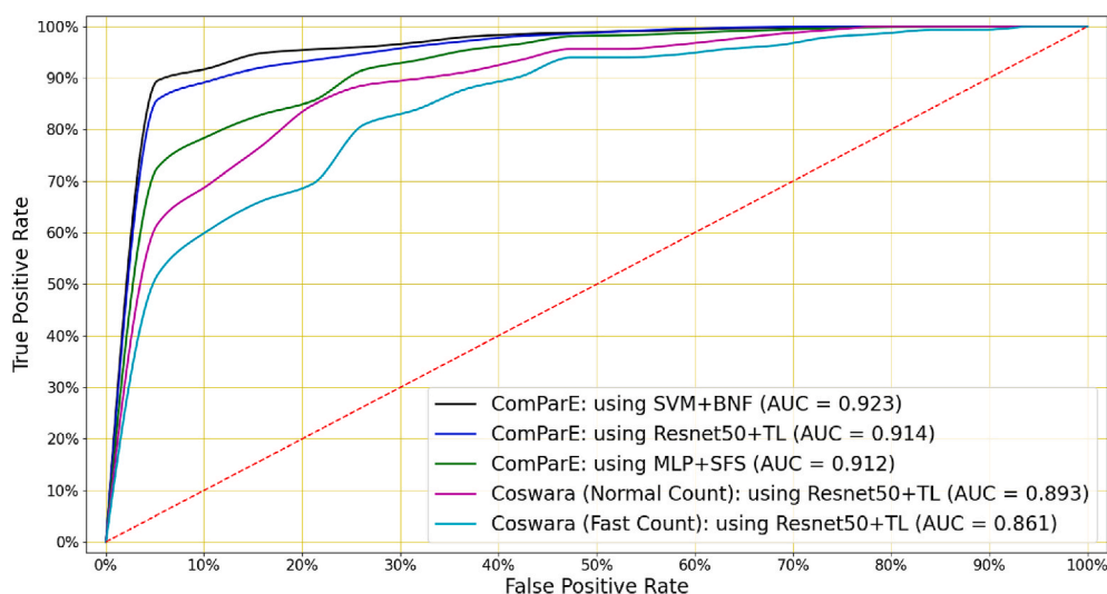
Fig. 7. COVID-19 speech classification: An SVM classifier using bottleneck features (BNF) achieved the highest AUC of 0.923 when classifying COVID-19 speech in ComParE dataset. A Resnet50 trained by transfer learning achieves a slightly lower AUC of 0.914. Speech (normal and fast) in the Coswara dataset can be used to classify COVID-19 with AUCs of 0.893 and 0.861 respectively using a Resnet50 trained by transfer learning.
