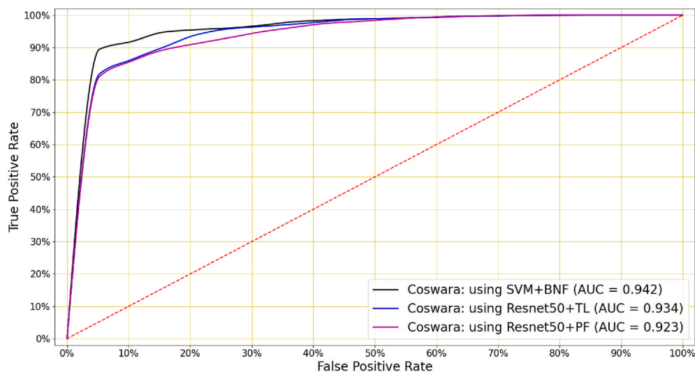
Fig. 6. COVID-19 breath classification: An SVM classifier using bottleneck features (BNF) achieved the highest AUC of 0.942 when classifying COVID-19 breath. The Resnet50 with and without the transfer learning has achieved AUCs of 0.934 and 0.923 respectively, with higher \sigma_{AUC} for the latter (Table 7).
