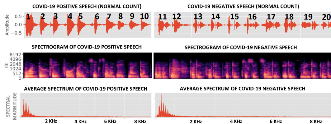
Fig. 2. Pre-processed speech (counting from 1 to 20 at a normal pace) from both COVID-19 positive and COVID-19 negative subjects in the Coswara dataset. In contrast to breath (Fig. 1), the spectral energy in this speech is concentrated below 1 kHz.
