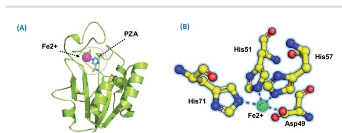
Fig. 1 (A) PZA-bound structure of pncA. (B) Binding of \text{Fe}^{2+} and its coordinated residues.
