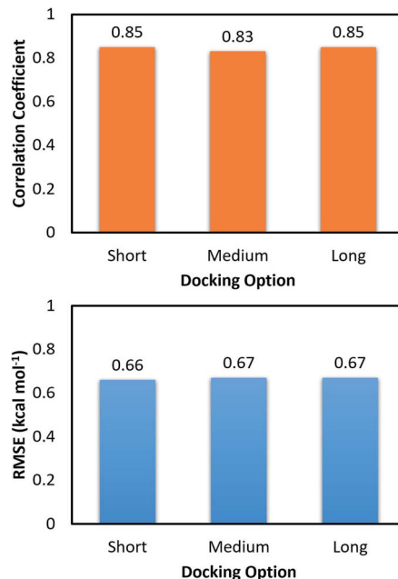
Fig. 4 Correlation and RMSE values between docking binding affinity of ligands to monomeric and dimeric forms of SARS-CoV-2 Mpro.
