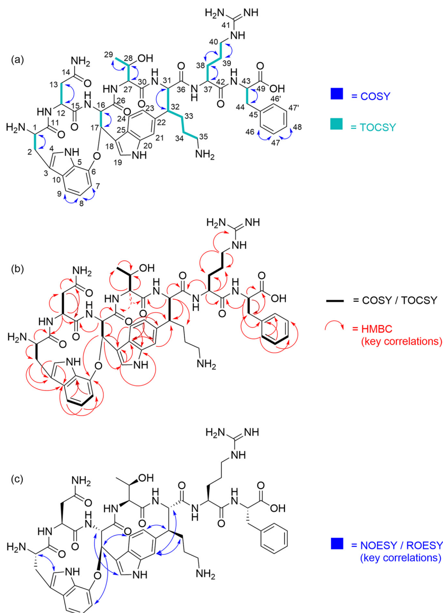
FIG 3 (a) Correlation spectroscopy (COSY) and total correlation spectroscopy (TOCSY) correlations, (b) key heteronuclear multiple-bond coherence (HMBC) correlations, and (c) key nuclear Overhauser effect spectroscopy (NOESY) and rotating-frame nuclear Overhauser effect spectroscopy (ROESY) correlations of darobactin B.
