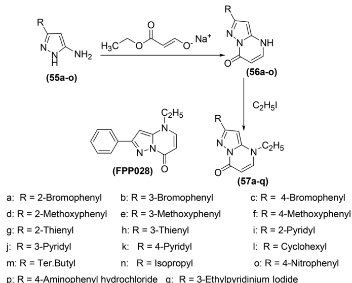
Scheme 24 Synthesis of pyrazolo[5,4-b]pyrimidin-7-ones (57a–q).
