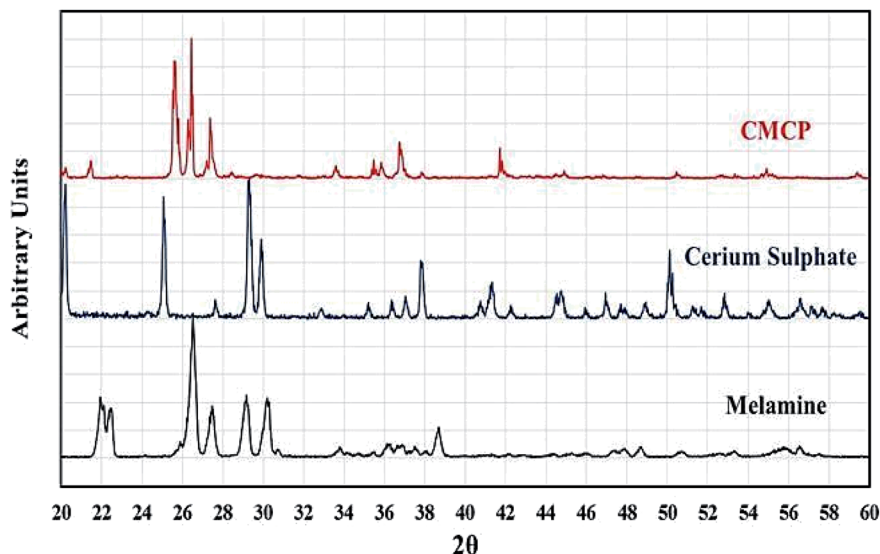
Fig. 3 XRD patterns of CMCP, cerium sulfate ( \text{Ce}_2(\text{SO}_4)_3 ), and melamine.
