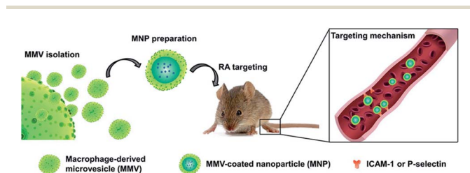
Fig. 6 Schematic illustration of MMV-coated nanoparticle (MNP) targeting sites of RA. MNP could target sites of RA through ICAM-1 or P-selectin adhesion. 62 Adapted with permission from ref. 62 (copyright 2019, American Chemical Society).
