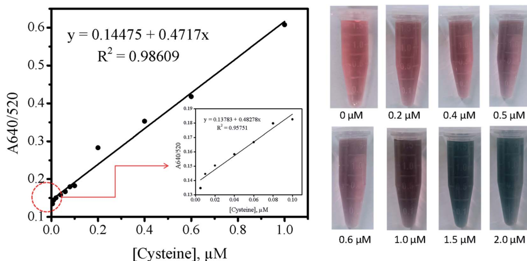
Fig. 8 The absorbance ratio of A_{640/520} (nm/nm) for the AuNPs–Cu 2+ sensing system at pH 7 over the concentration range (0.005–1.0 \mu\text{M} ). The inset shows the magnified representation of A_{640/520} ratio from 0.005 \mu\text{M} to 0.1 \mu\text{M} . The right pictures show the progressive colorimetric changes of the AuNPs–Cu 2+ sensing system with increasing Cys concentration (0–2.0 \mu\text{M} ).
