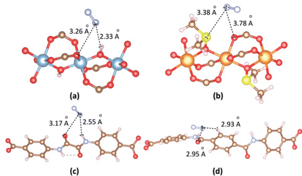
Fig. 10 The main adsorption sites of N 2 in the vicinity of (a) [Al 2 (OH) 2 (CO 2 ) 4 ] ∞ cluster, (b) {Mg 2 [OS(CH 3 ) 2 ] 2 (CO 2 ) 4 ] ∞ cluster, (c) ODA 2- linker and (d) TDA 2- linker.
