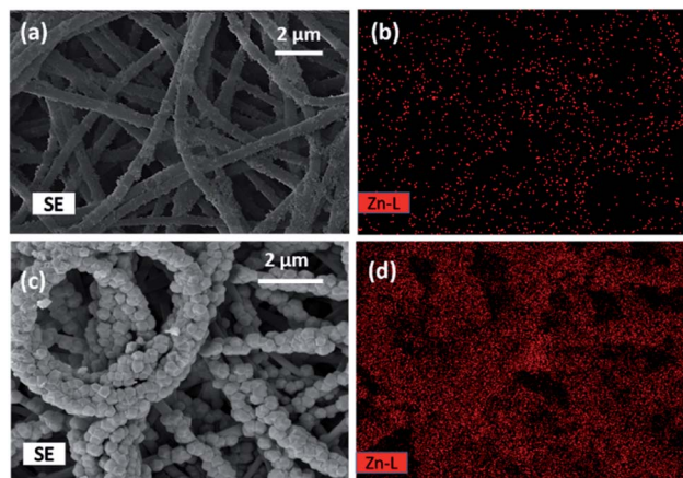
Fig. 3 SEM micrographs and EDS mapping of Zn(OH)_2 /PAN nanofibers with (a) SEM microstructure, (b) distribution of Zn (in the top); and of ZIF-8/PAN-90 nanofibers with (c) SEM microstructure and (d) distribution of Zn (in the bottom).
