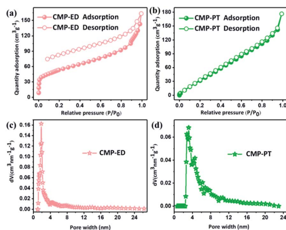
Fig. 4 Nitrogen adsorption and desorption isotherms (a) and (b), and distribution of pore size of CMP foams (c) and (d).
