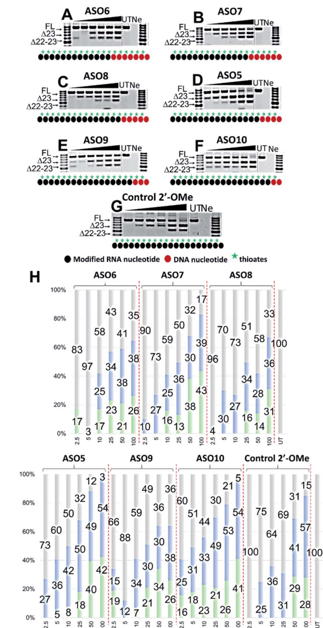
Fig. 3 RT-PCR with sequence visualisation (A–G) and densitometry analysis (H) of RNA prepared from H2K mdx mouse myotubes transfected with ASO6 (A), 7 (B), 8 (C), 5 (D), 9 (E), 10 (F) and control 2'-O-Me ASO (G). The triangles above the gel image indicate increasing ASO concentration (2.5, 5, 10, 25, 50 and 100 nM); FL (full-length) = 901 bp, represented in grey color; Δ23 (exon-23 skipped) = 688 bp, represented in blue color; Δ22-23 (exons-22 + 23 skipped) = 542 bp, represented in green color; UT = untreated, Ne = negative control.
