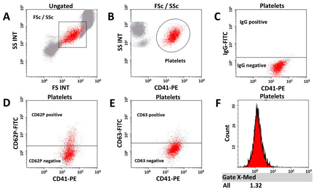
Figure 6. Expression of PLT activation markers. (A) Preliminary PLT gating based on morphological properties—forward scatter (FS) and side scatter (SS). (B) Precise PLT gating based on CD41 expression. (C) Positive threshold setting based on isotype control (IgG) expression. (D) Evaluation of CD62P activation marker expression. (E) Evaluation of CD63 activation marker expression. (F) Histogram to determine the median MFI of the marker of interest. This is the representative protocol for EDTA control blood samples.
