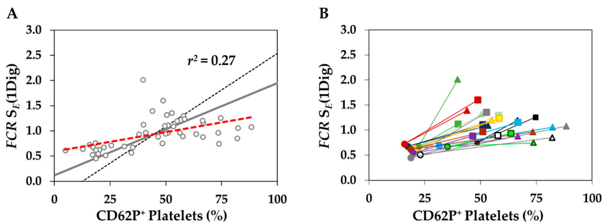
Figure 8. The relationship between PLT activation and mitochondrial respiration of PLT in the S-pathway. Respiration of permeabilized PLT in the S-pathway ( S_E , expressed as FCR normalized for ET capacity E of living cells, FCR = S_E/E ), and PLT activation expressed as a percentage of CD62P positive cells. (A) Regression analysis according to [49] where the red dotted line represents ordinary Y/X regression and the black dotted line represents ordinate projection of abscissal regression with inverted parameters X/Y , and the grey line represents mean regression line; r^2 is independent of axes inversion. (B) Data points for individual blood donors are connected by a full line from DC (triangles) to PA (circles) and WA (squares); each color indicates a different donor.
