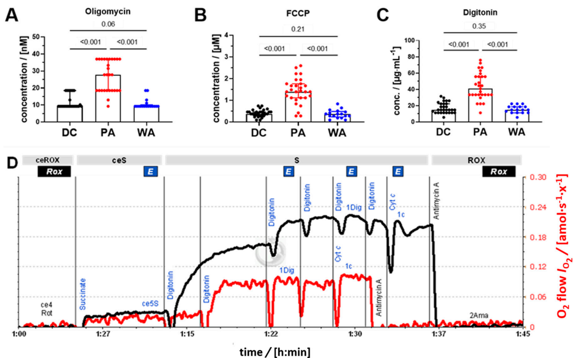
Figure 4. Effect of isolation methods on the inhibitory concentration of oligomycin, and optimum concentrations of uncoupler FCCP and digitonin. (A) Adenosine triphosphate (ATP)-synthase inhibitor oligomycin. (B) Uncoupler FCCP. (C) Mild detergent digitonin for plasma membrane permeabilization. (D) Representative trace of the viability module of the SUIT protocol. DC (black) and PA (red). Oxygen flow per cell I_{O_2} [ \text{amol}\cdot\text{s}^{-1}\cdot\text{x}^{-1} ]. One-way ANOVA with multiple comparison test (Tukey), p values are shown above their respective pairwise comparison bar.
