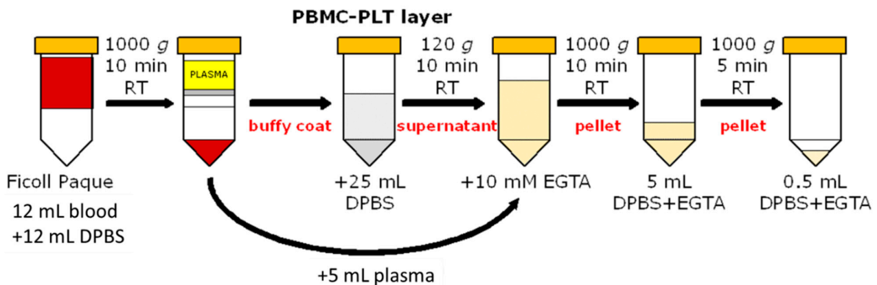
Figure 1. Scheme of platelets (PLT) preparation using density gradient centrifugation (DC). From the first centrifugation of whole blood with Ficoll-Paque™ to the final pellet, which was resuspended in Dulbecco's phosphate-buffered solution (DPBS) and ethylene glycol-bis (2-aminoethyl ether)- N,N,N',N' -tetra-acetic acid (EGTA) at room temperature (RT). The PLT suspension was counted (10 times diluted) and added to the O2k-chamber at a final cell concentration of 200 \times 10^6 \times \text{mL}^{-1} . PBMC, peripheral blood mononuclear cell.
