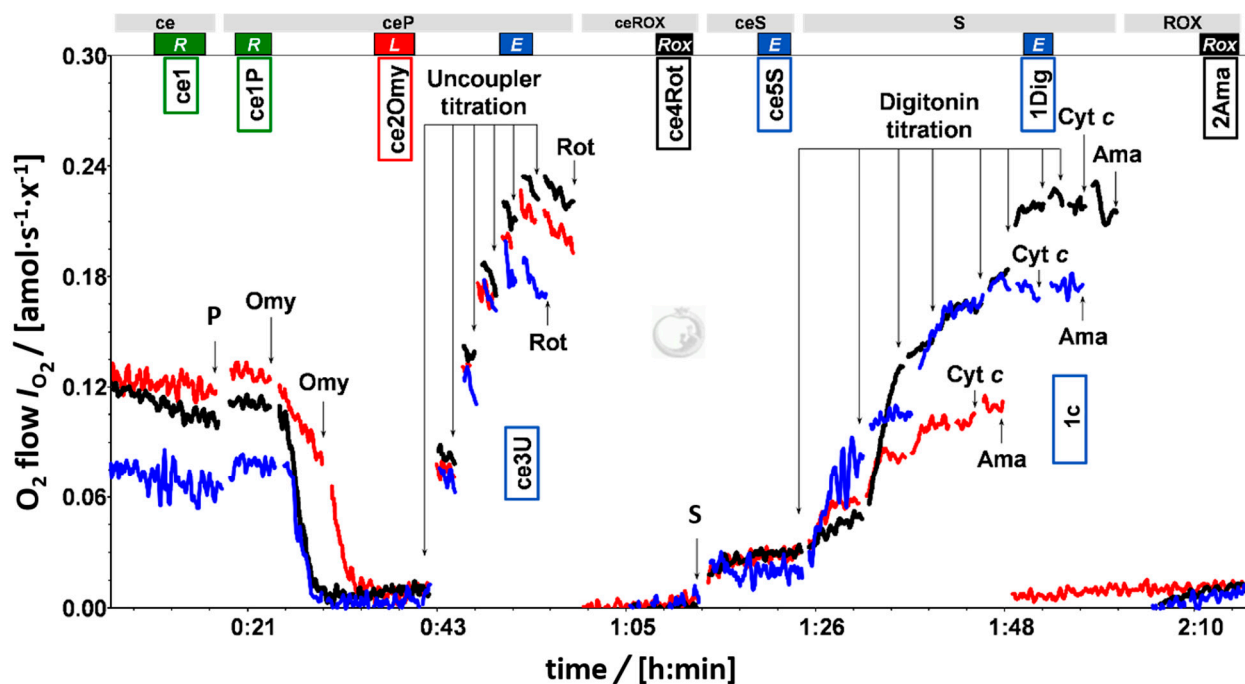
Figure 2. Representative traces of PLT respiration of DC (black), platelet apheresis (PA; red), and washed apheresis (WA; blue) samples. Oxygen flux per cell, I_{O_2} [ \text{amol}\cdot\text{s}^{-1}\cdot\text{x}^{-1} ]. Coupling control and cell viability (CCV) protocol with living cells (ce1), pyruvate addition (ce1P), oligomycin titration (10 to 40 \text{nmol}\cdot\text{L}^{-1} ; ce2Omy), uncoupler titration of carbonyl cyanide 4-(trifluoromethoxy)phenylhydrazone (FCCP) at 0.1 \mu\text{mol}\cdot\text{L}^{-1} steps (ce3U). Rotenone for residual oxygen consumption (ce4Rot; 1 \mu\text{mol}\cdot\text{L}^{-1} ROX). Cell viability test in the CCV protocol: succinate addition (ce5S; 20 \text{mmol}\cdot\text{L}^{-1} ) with digitonin titration (1Dig). Cytochrome c test (1c; 10 \mu\text{mol}\cdot\text{L}^{-1} ) and antimycin-A addition for Rox (2Ama; 2.5 \mu\text{mol}\cdot\text{L}^{-1} ).
