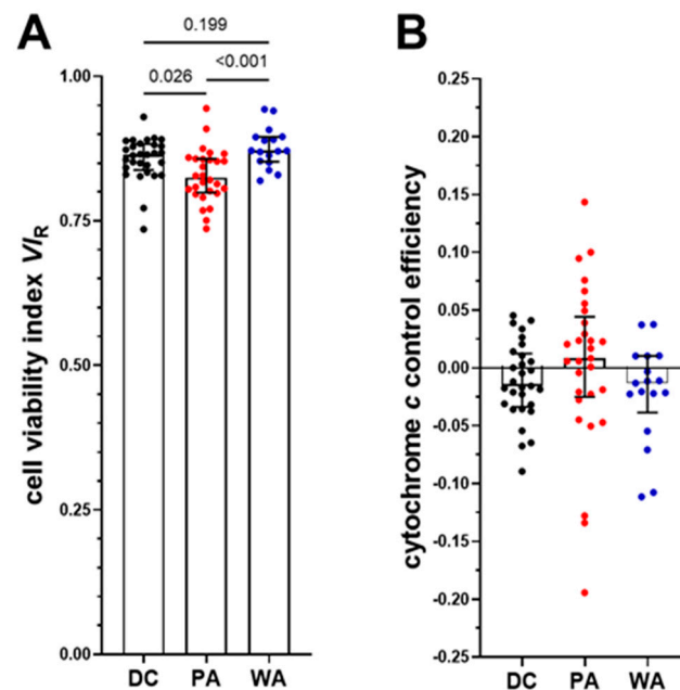
Figure 5. Effect of isolation methods and media on PLT viability. (A) Respirometric cell viability index ( VI_R ) of PLT isolated by DC (black symbols), PA (red symbols), and WA (blue symbols). The respirometric cell viability index is VI_R = 1 - (J_{ce5S} - J_{ce4Rot}) / (J_{1Dig} - J_{2Ama}) [34]. (B) Cytochrome c control efficiency expresses the integrity of the outer mitochondrial membrane and is calculated as a change in respiration after the addition of cytochrome c , j_c = (J_{1c} - J_{1Dig}) / (J_{1c} - J_{2Ama}) [3,34]. Titration steps (ce4Rot, ce5S, 1Dig, and 1c) are depicted in Figure 2. One-way ANOVA with mixed-effects model, p values are shown above their respective pairwise comparison bar.
