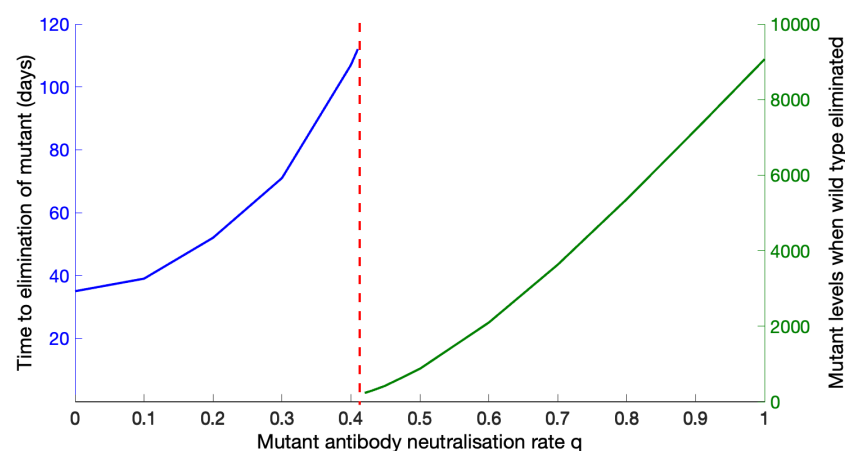
Figure 7. Sensitivity of the outcome to the mutant antibody-neutralisation rate, q . Below q = 0.41 , elimination of the mutant is possible; above q = 0.41 , elimination is no longer possible, and the mutant levels increase as q increases.
