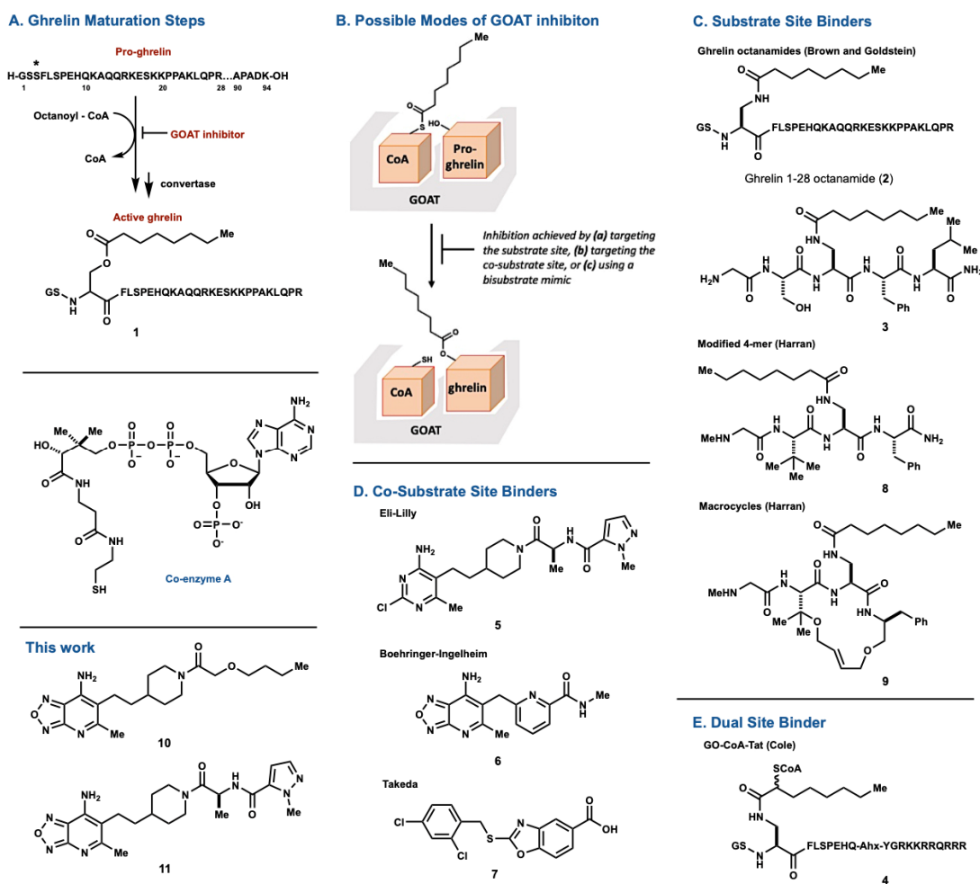
Figure 1. (A) GOAT-catalyzed octanoylation of pro-ghrelin is a critical part of ghrelin maturation. GOAT is weakly inhibited by its reaction product, acyl ghrelin (1), and more potently by analog 2, wherein Ser-3 is replaced by diaminopropionic acid (DAP). Systemic inhibition of GOAT is expected to reduce circulating acyl-ghrelin levels, leading to improved insulin response to glucose challenge. (B) GOAT inhibition can be achieved by targeting either the substrate or co-substrate site, or by targeting both sites with a “bisubstrate” mimic. (C–E) Known inhibitors of GOAT.
