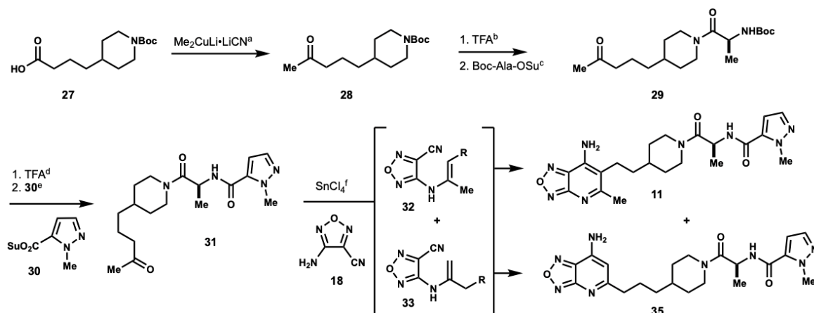
Scheme 2. (a) CuCN (5 eq.), Et 2 O (0.6 M), MeLi (1.6M in Et 2 O; 10 eq.), 0 °C; 27 (1 eq.), Et 2 O (0.2 M), 71%; (b) CH 2 Cl 2 (0.07 M), trifluoroacetic acid (TFA) (10% v/v ), 0 °C; (c) Boc-Ala-OSu (1.1 eq.), DIPEA (3.1 eq.), MeCN (0.2 M), 0 °C, 50% over two steps; (d) CH 2 Cl 2 (0.07 M), trifluoroacetic acid (TFA) (10% v/v ), 0 °C; (e) 30 (1 eq.), DIPEA (3 eq.), MeCN (0.2 M), 0 °C, 72% over two steps; (f) 18 (1 eq.), SnCl 4 (2 eq.), toluene (0.2 M), reflux.
