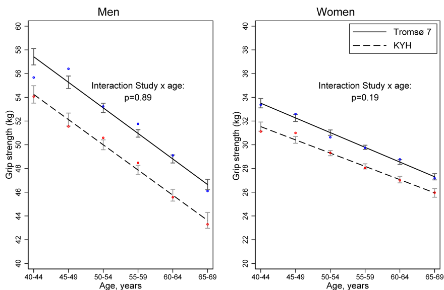
Figure 1 Mean grip strength (kg) (95% confidence intervals) by age and study in men and women. Estimated in sex-specific linear regression models including age, study, and an age by study interaction ( N = 9431 ). *Dots are unadjusted observed means (blue for Tromsø 7 and red for Know Your Heart Study)
