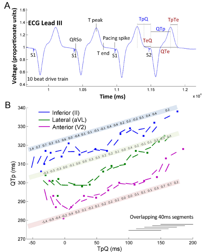
Figure 3 Derivation of Regional Restitution Instability Index (R2I2) and Peak ECG Restitution Slope (PERS). (A) Stimulation protocol demonstrating the fiducial points of T_{\text{peak}}-Q and QT_{\text{peak}} (blue) which are required to plot on the restitution curve (B) gradients are fitted for each 40 ms overlapping least square segment. The mean of the SD of gradient differences from the mean gradient is taken as the R2I2. The mean of the peak restitution curve slope is calculated to be the PERS value (reproduced with permission from Nicolson 2014). 19
