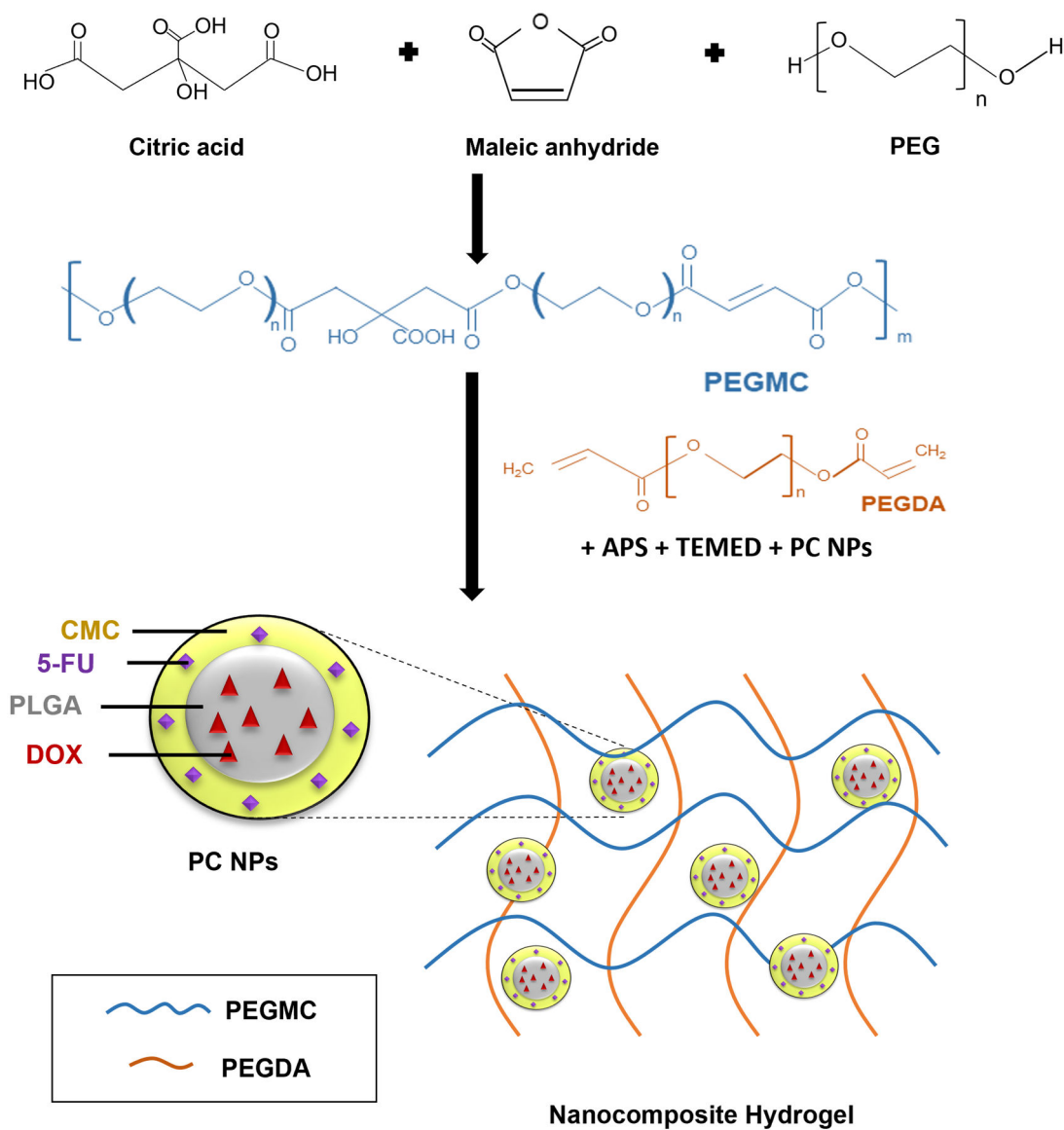
Figure 1: Schematic illustration of the synthesis and use of PEGMC polymer to form the NCH system containing pH-responsive PC NPs.
