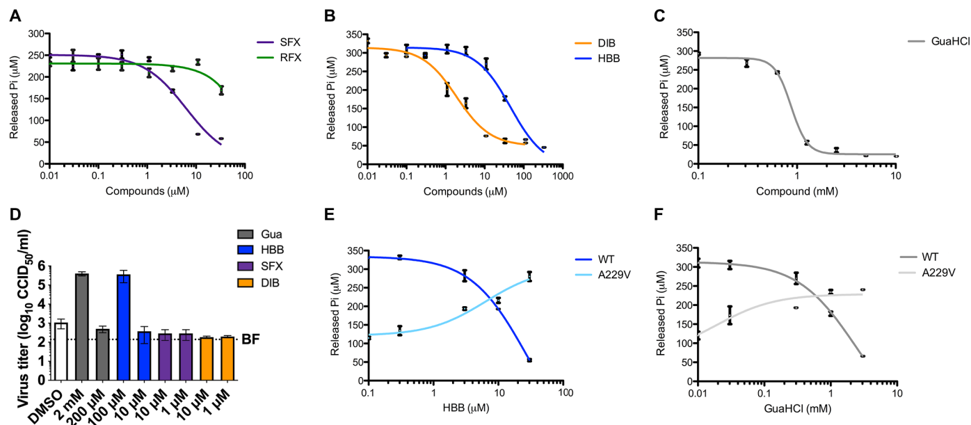
Fig. 4. 2C inhibitors reduce the ATPase activity of 2C and have antiviral effect. (A to C) Effects of SFX and RFX (A), dibucaine (DIB) and [2-(alpha-hydroxybenzyl)-benzimidazole] (HBB) (B), or guanidium hydrochloride (GuaHCl) (C) on 2C-dependent ATPase activity. (D) Replication of CV-B3 containing the A229V 2C mutation in the presence of GuaHCl, HBB, SFX, or DIB (or a nonrelated replication inhibitor, BF738735, which targets a host lipid kinase). At 8 hours after infection, cells were freeze-thawed, and virus titers of lysates were determined. (E and F) Comparison of ATPase activity of WT 2C and the A229V mutant in the presence of HBB (E) and GuaHCl (F). Experiments shown in (A) to (C), (E), and (F) were performed twice, each time in technical duplicates. The experiment in (D) was performed in biological triplicates.
