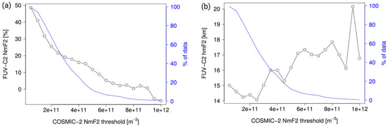
Figure 6. Relative N_mF_2 (a) and absolute h_mF_2 values (b) with respect to C2. The x -axis represents the C2 N_mF_2 threshold used to compute the mean relative difference, that is, all measurements for which N_mF_2 is larger than this given threshold are participating to the average plotted on the y -axis. The right axis represent the fraction of the measurements participating to each data point.
