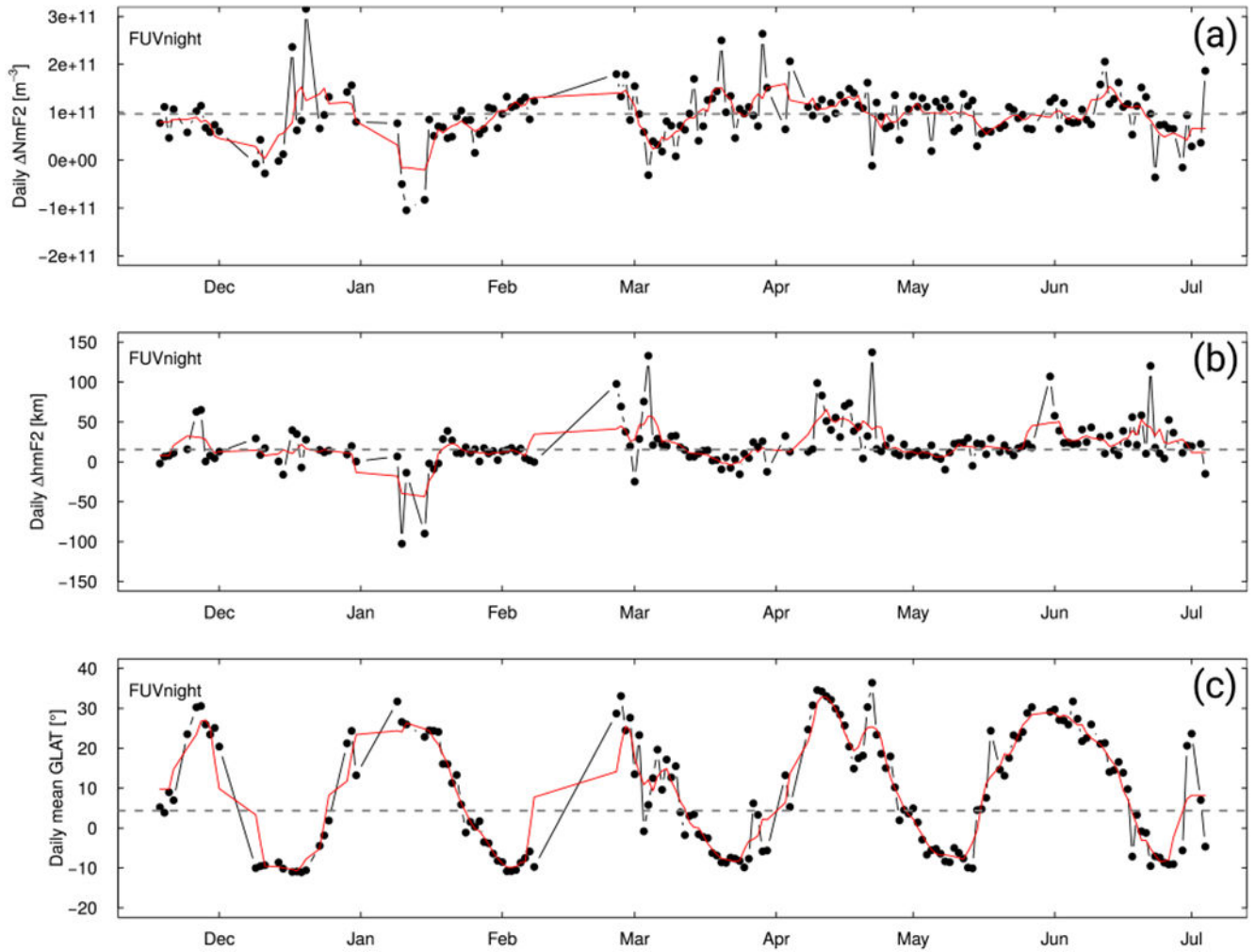
Figure 8. C2 comparison. Time series of FUV daily mean N_mF_2 , h_mF_2 and geographic latitude. The corresponding 5-day running mean is plotted with the solid red line. The mean values for the whole data sets are plotted with the dashed gray line and correspond to the values appearing in Table 1.
