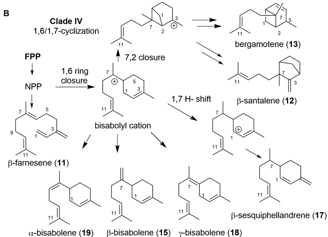
FIG 8 Putative enzymatic conversion of GPP (A) and FPP (B) by terpene cyclase TTC15-T153.
