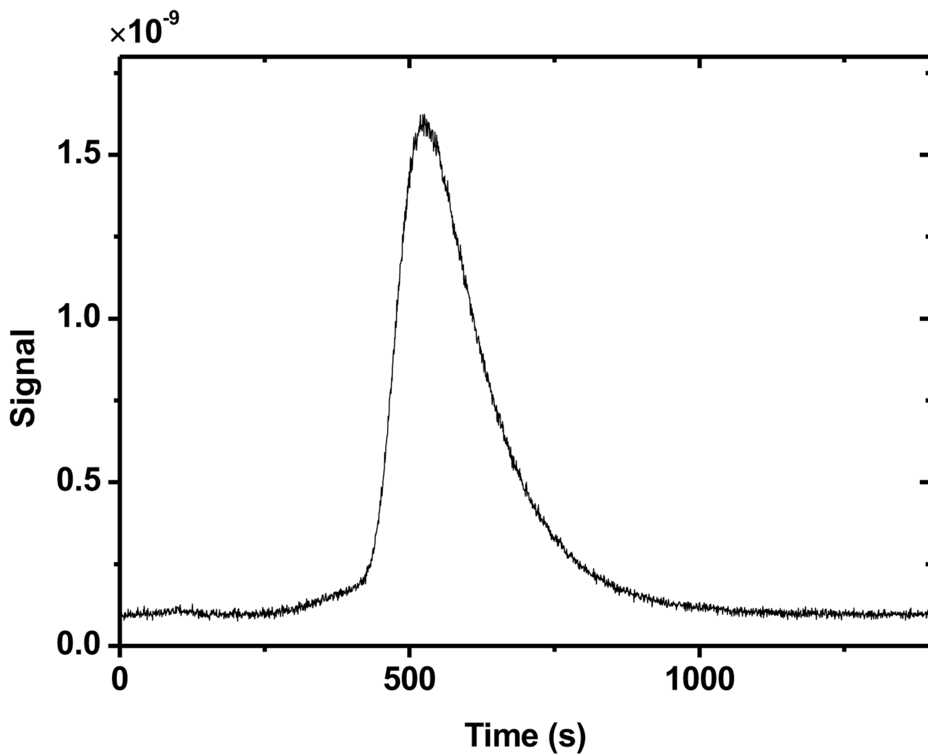
Fig. 4. A representative current signal (amps) from the mass spectrometer for 4.57 \mu\text{mol} of \text{H}_2 dissolved in deionized water.
