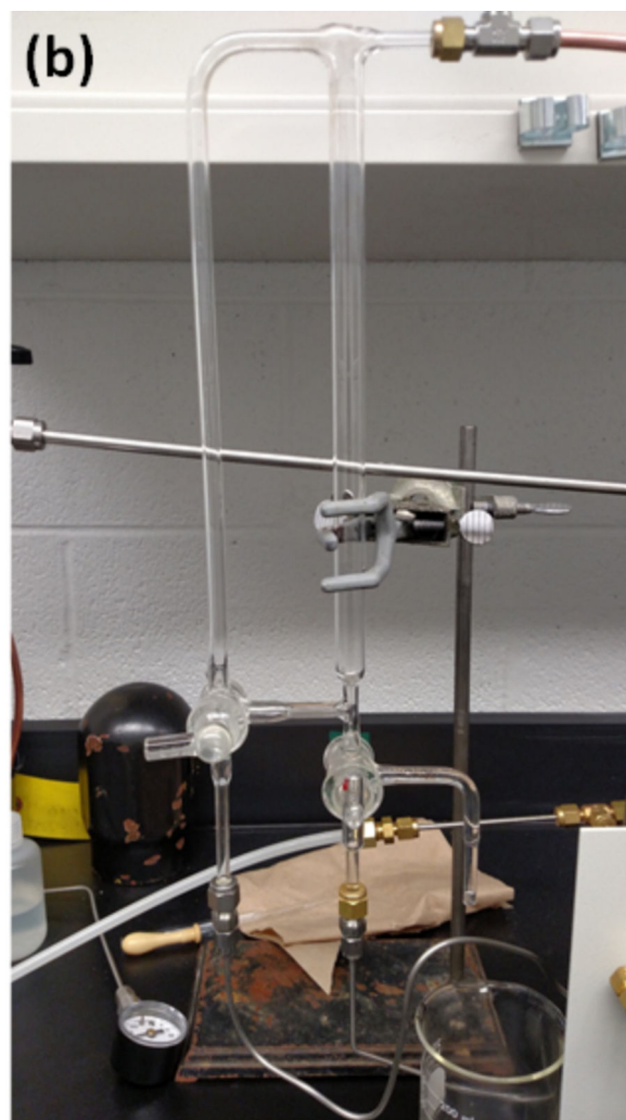
Fig. 1. A block diagram (a) of the experimental set-up for the flow system to irradiate and collect samples of borated water and an image of the glass sparging apparatus (b) used to collect the irradiated water and sparge out H 2 from the water sample.
