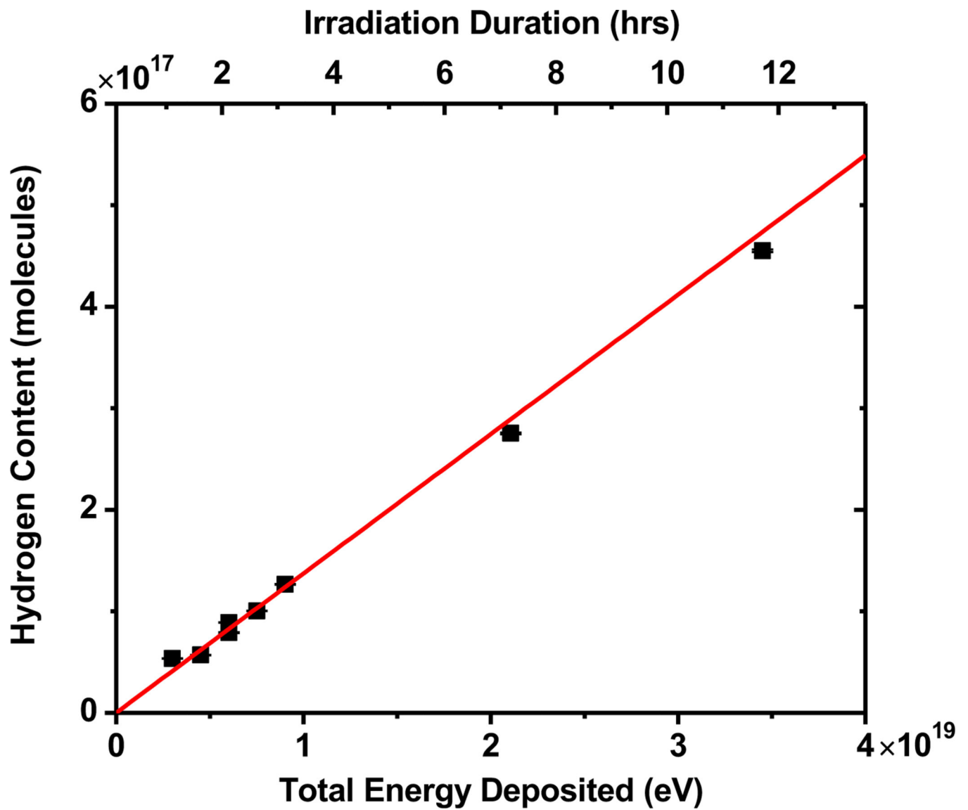
Fig. 6. Relationship between the molecules of H_2 obtained from sample versus total energy deposited in the sample via the B^{10}(n,\alpha)^7Li reaction.
