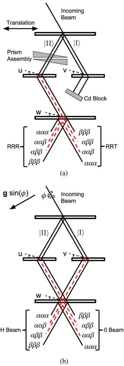
FIG. 4. (a) Our experimental setup used to measure intrinsic misalignments in an interferometer. (b) The Mach-Zehnder neutron interferometer geometry used in the COW experiments. Here the direction of gravity is denoted by g \sin(\phi) , where \phi is the interferometer tilt about the incoming beam axis.
