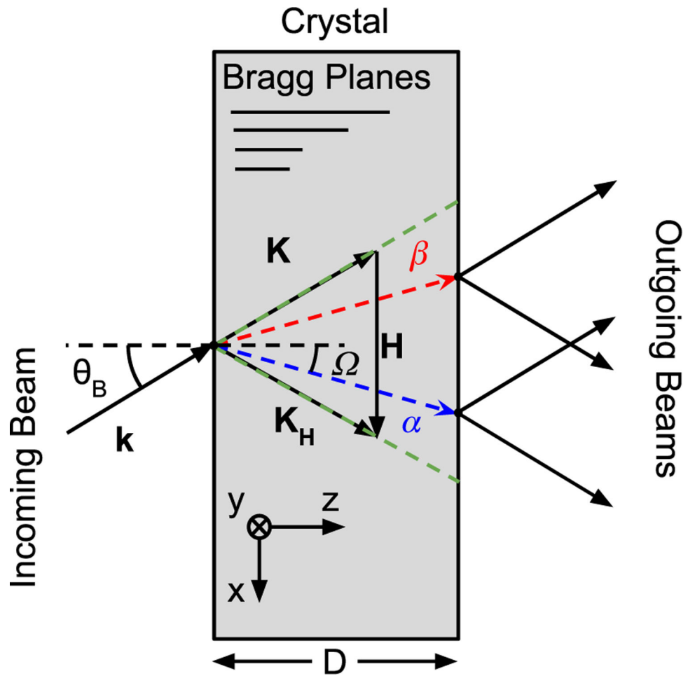
FIG. 2. An incoming momentum state |k\rangle excites two degenerate, \{\alpha, \beta\} , states within the crystal. These two states become spatially separated according to the microradian misalignment of |k\rangle from the exact Bragg condition. Each incoming neutron wave packet fills the entire Borrmann fan (outlined by green dashed lines).
