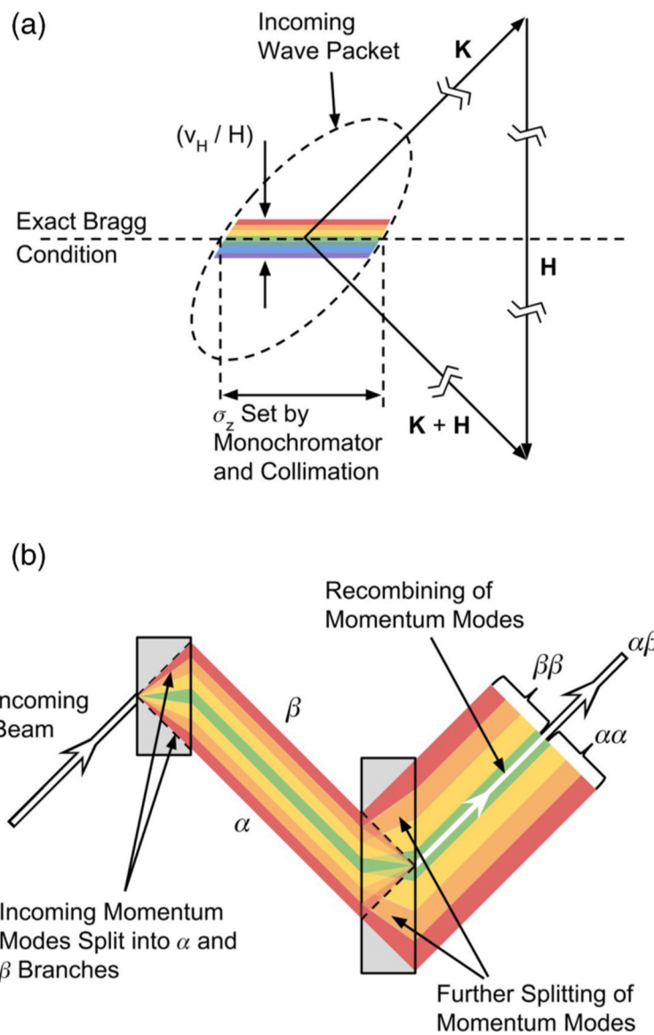
FIG. 3. Dynamical phases in a two-crystal geometry. (a) Momentum-space depiction, with the component of k along H selected by the crystal colored. The magnitude of the crystal’s angular acceptance relative to the spread of the wave packet in phase space is greatly exaggerated for clarity. (b) Coherent recombination is dependent on the precise alignment of the crystals and a uniform potential between and within the diffracting crystals. Only the infrared deviations from Bragg are shown; the ultraviolet deviations follow the same pattern.
