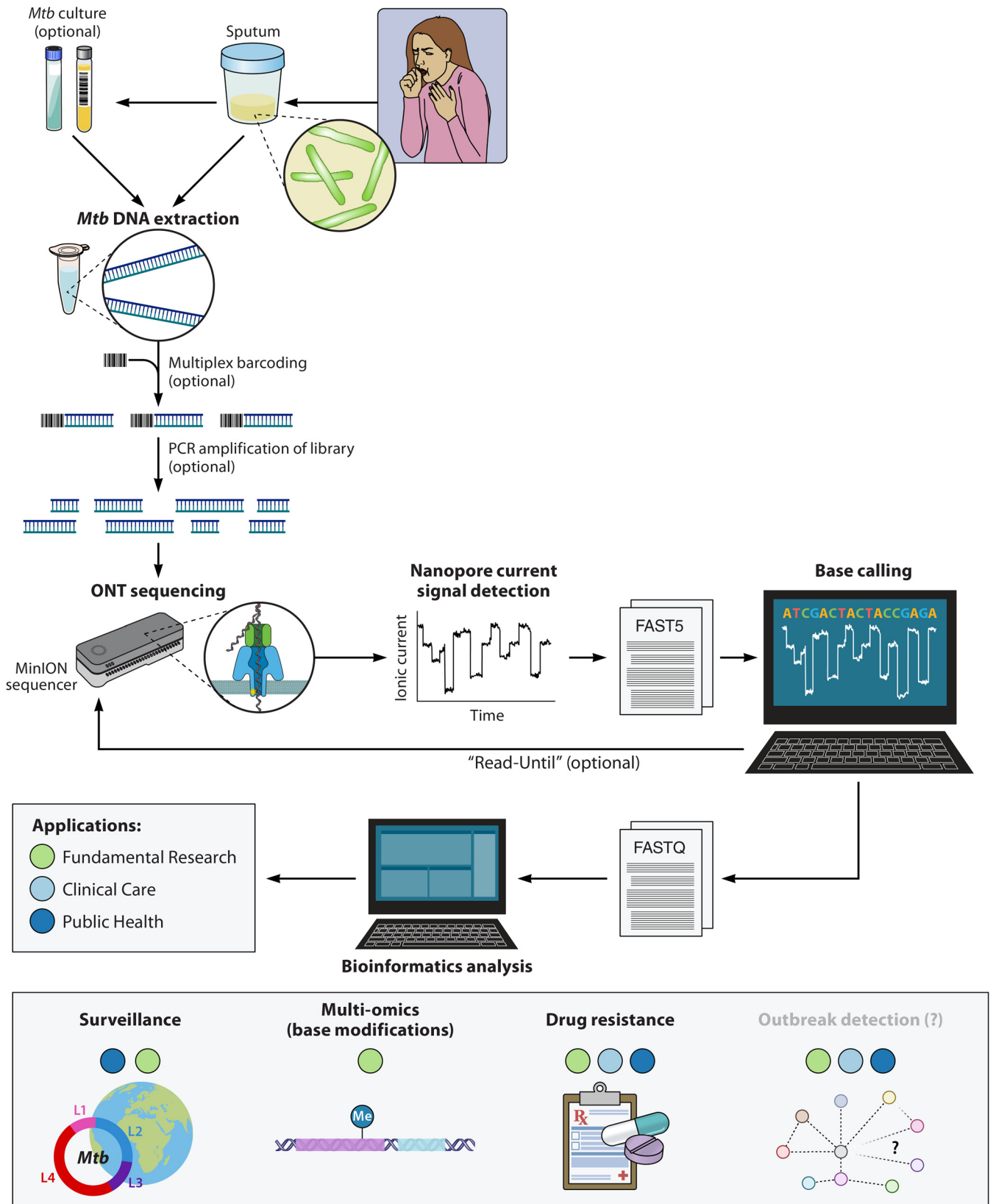
FIG 1 Overview of the Mycobacterium tuberculosis sequencing approach using Oxford Nanopore Technologies sequencing platform. After DNA extraction, usually from cultured M. tuberculosis but, in some cases, directly from clinical specimens, ONT library preparation is done, which may include barcoding and/or PCR amplification of the sequence library. The prepared library is loaded on the flow cell and inserted in the sequencer that is connected to a (Continued on next page)
