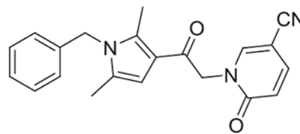
CYM-5520
