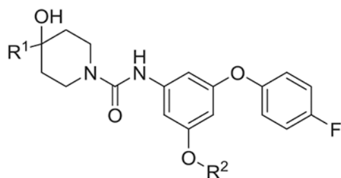
1,3-bis(aryloxy)benzene derivatives
