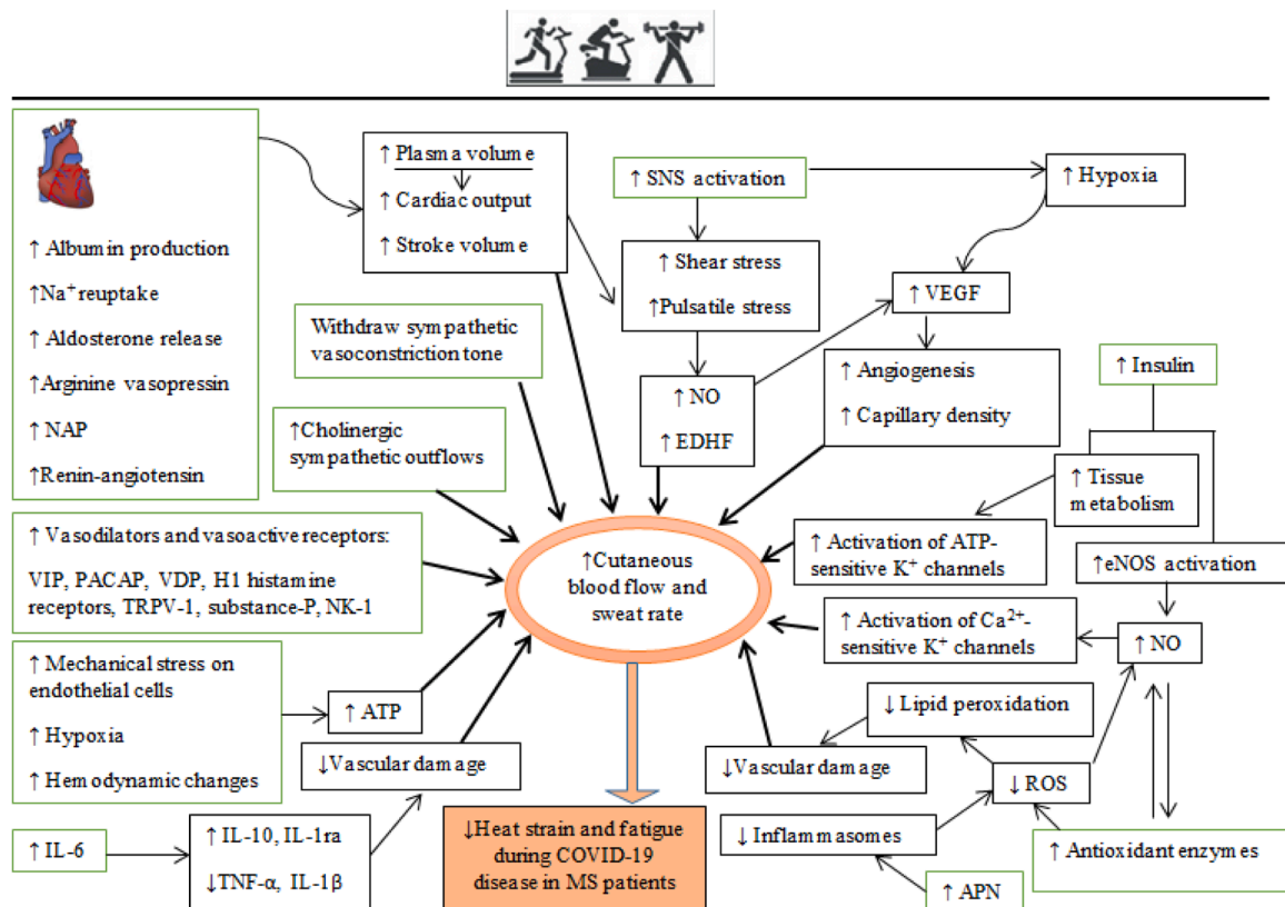
Fig. 2. Schematic diagram of physical exercise-induced adaptations in improving thermal management. The green rectangles represent the main adaptations induced directly by regular physical exercise that are associated with secondary adaptations (in black rectangles). The bold arrows show the main adaptations; oval circles indicate increased cutaneous blood flow resulting from vascular adaptations. Na + , sodium; NAP, natriuretic atrial peptide; VIP, vasoactive intestinal peptide; PACAP, pituitary adenylate cyclase-activating polypeptide; VDP, vascular-dilating prostanoids; TRPV-1, transient receptor potential vanilloid type 1; NK-1, neurokinin-1; NO, nitric oxide; EDHF, endothelial-derived hyperpolarizing factor; VEGF, vascular endothelial growth factor; ROS, reactive oxygen species; APN, adiponectin.
