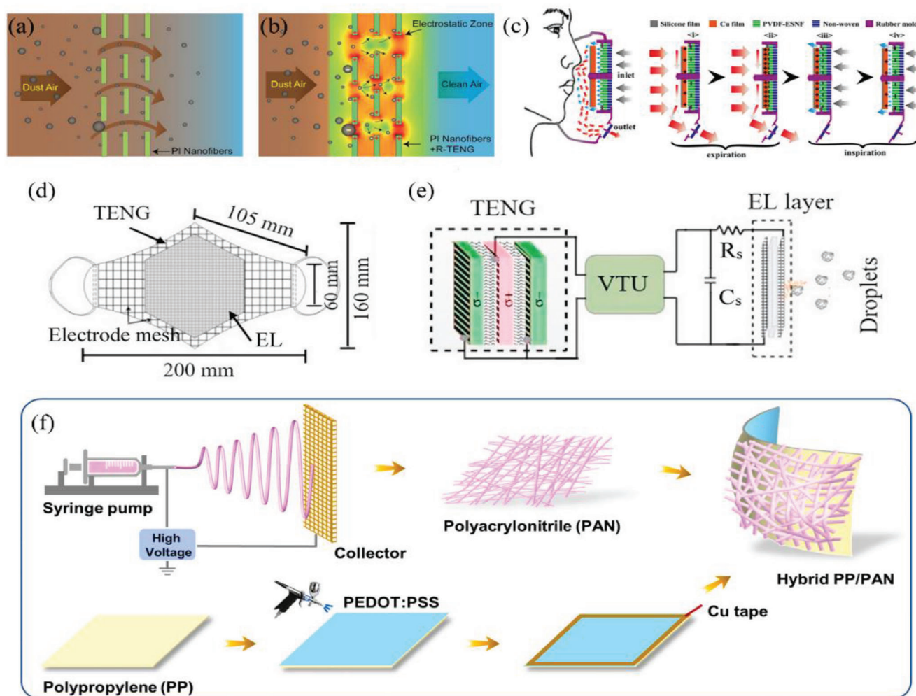
Figure 13. The schematic illustration of different face masks integrated with triboelectric nanogenerator (TENG). a,b) show the filtration performance before and after applying rotating triboelectric nanogenerator in air filter by Gu et al., respectively. a,b) Adapted with permission. [289] Copyright 2017, American Chemical Society. c) The structure of respiratory triboelectric nanogenerator for the self-powered electrostatic absorption face mask by Liu et al. Adapted with permission. [290] Copyright 2018, American Chemical Society. d) The proposed design of triboelectric self-powered mask and e) The diagram of face mask with the TENG by Ghatak et al. d-e) Reproduced with permission. [292] Copyright 2021, Elsevier. f) Schematic illustration of the fabrication process of a new nano/micro fibrous hybrid mask. Reproduced with permission. [287] Copyright 2021, Elsevier.
