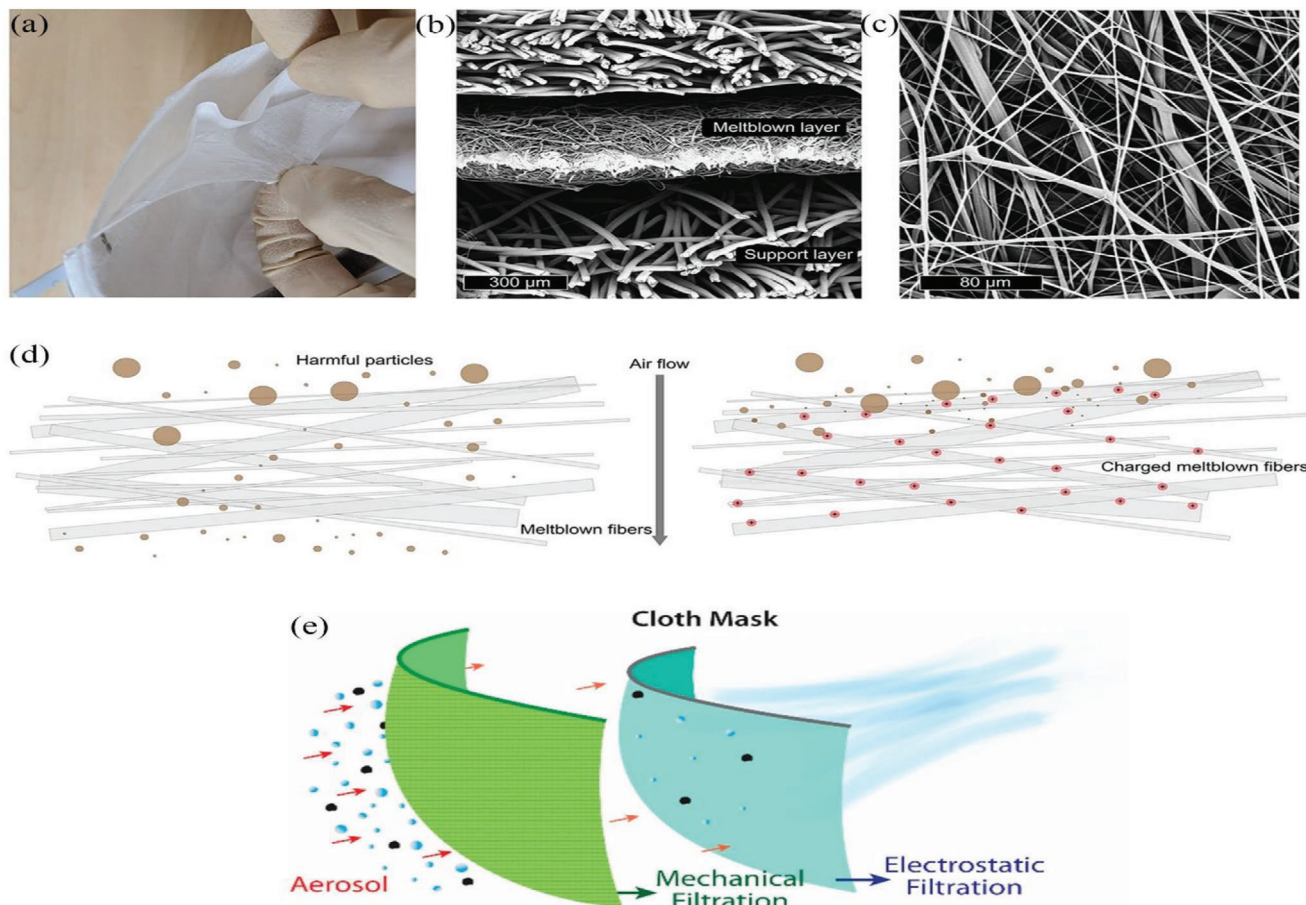
Figure 4. Structure diagram of N95 respirators. a) Peeling apart a representative N95 respirator reveals multiple layers of nonwoven materials. b) Scanning electron microscope (SEM) cross-section image reveals that the middle meltblown layer has finer fibers with thickness around 300 \mu\text{m} . c) SEM image of meltblown fibers reveals a complicated randomly oriented network of fibers with diameters \approx 1\text{--}10\ \mu\text{m} . d) Schematic illustration of meltblown fibers (left) without and (right) with electret charging. In the left figure, smaller particles are able to pass through to the user, but they are electrostatically captured in the case of an electret (right). a-d) Reproduced with permission. [5] Copyright 2020, American Chemical Society. e) Schematic illustration of homemade cloth masks obtained by combining different fabric materials. Reproduced with permission. [90] Copyright 2020, American Chemical Society.
