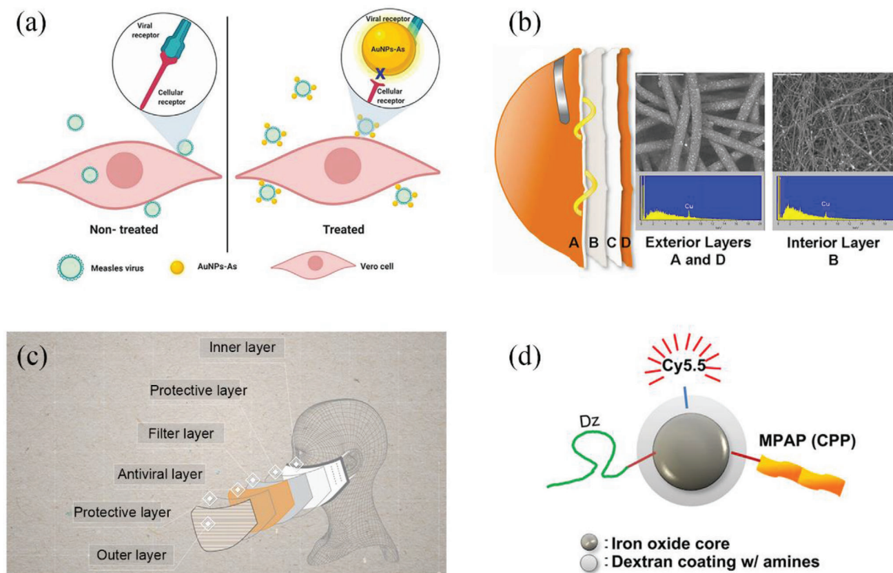
Figure 8. Some anti-microbial applications of metals and its derivatives. a) The antiviral schematic diagram of gold nanoparticles. Reproduced under the terms of the Creative Commons Attribution 4.0 International License. [174] Copyright 2019, The Authors. Licensee MDPI, Basel, Switzerland. b) N95 mask treated with CuO NPs has antiviral property to kill viruses retained by the mask without changing the physical barrier performance. Reproduced under the terms of the Creative Commons Attribution License. [190] Copyright 2010, Borkow et al. c) The structure diagram of CuMask+ provided by the Hong Kong Government. Reproduced with permission. [191] Copyright 2020, The Hong Kong Research Institute of Textiles and Apparel Limited (HKRITA). d) The working mechanism of a multifunctional iron oxide nanoparticle for DNAzyme delivery (Dz, DNAzyme; MPAP, myristoylated polyarginine peptide; Cy5.5, fluorescent dye; CPP, cell-penetrating peptide). Reproduced with permission. [197] Copyright 2012, Elsevier.
