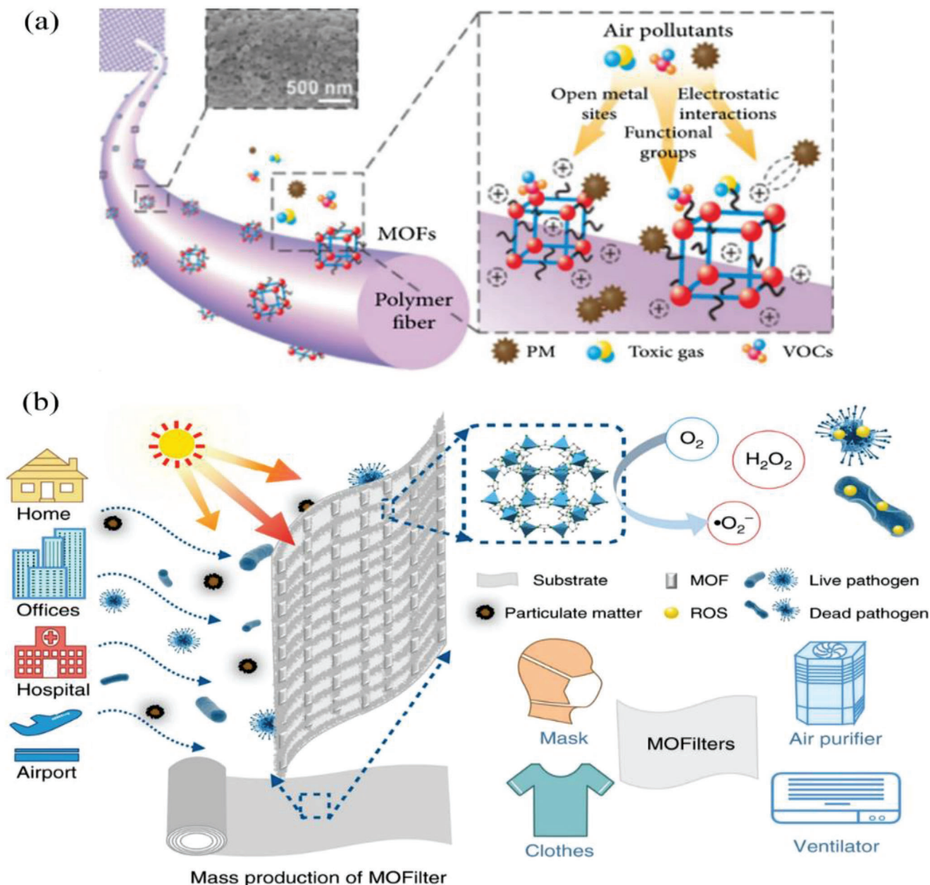
Figure 11. The mechanism diagram of MOF cleaning air. a) The surface of the MOF/polymer composite fiber. Reproduced under the terms of the Creative Commons Attribution 4.0 International License. [244] Copyright 2020 Ming Hui Chua et al. Exclusive Licensee Science and Technology Review Publishing House. b) The schematic of a metal-organic framework (MOF)-based filter for integrated air cleaning. Adapted under the terms of the Creative Commons Attribution 4.0 International License. [247] Copyright 20219, Springer Nature.
