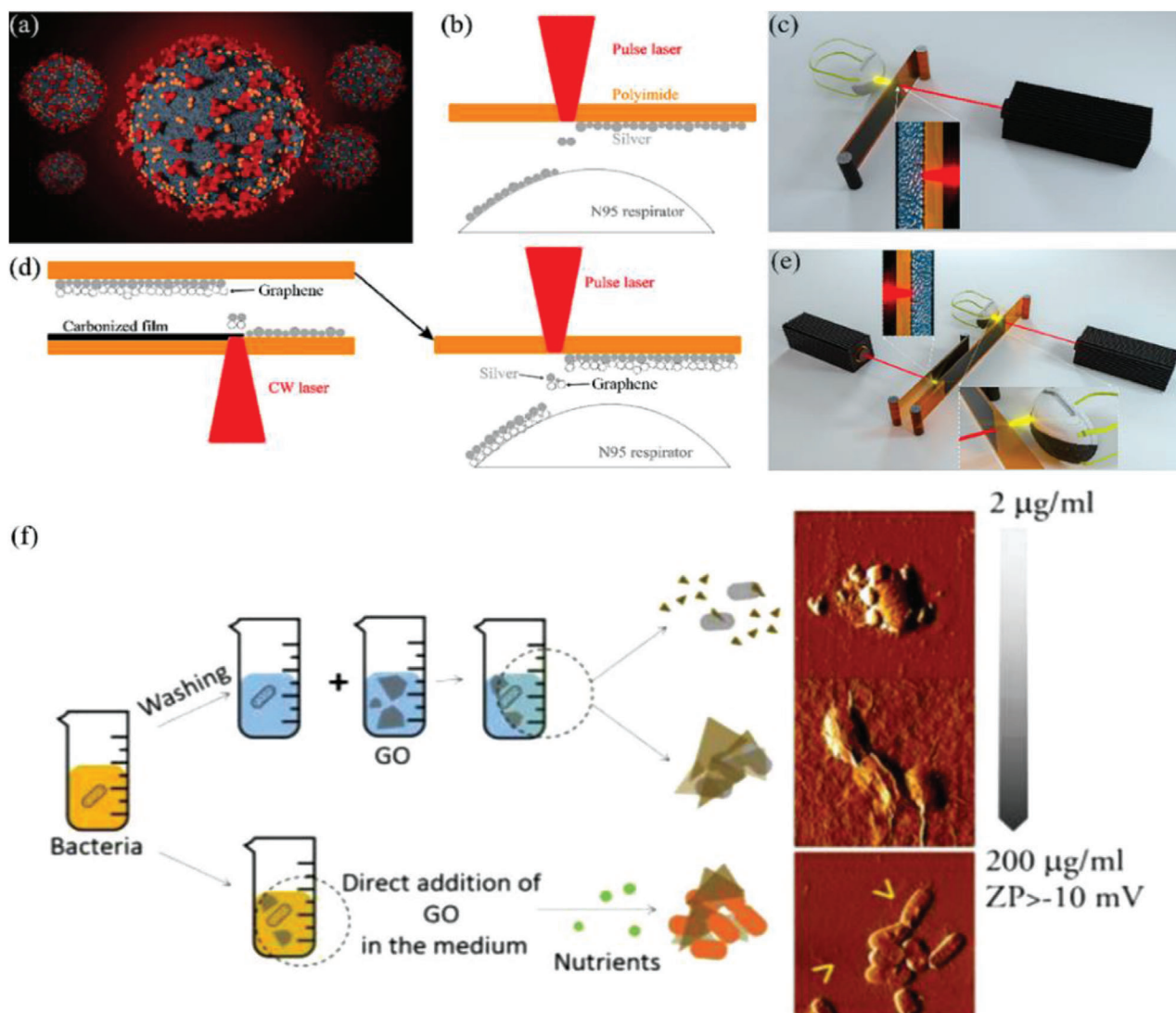
Figure 10. The fabrication processes of LIG-Ag NPs mask. a) Illustration of the SARS-COV-2 virus, b) M1 laser printing strategy, c) Illustration of the setup of the M1 laser printing method, d) M2 laser two-step laser printing strategy, e) Illustration of the setup of the M2 laser printing method. a-e) Reproduced with permission. [216] Copyright 2020, American Chemical Society. f) The antibacterial or growth-promoting effects on Staphylococcus aureus and Escherichia coli . Adapted with permission. [218] Copyright 2017, American Chemical Society.
