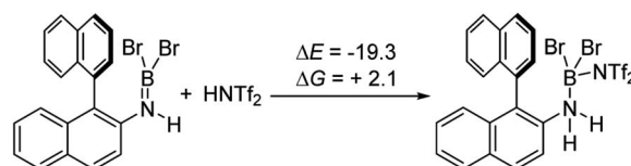
Scheme 7 Energy change on protonation with HNTf_2 ( kcal\ mol^{-1} ).
