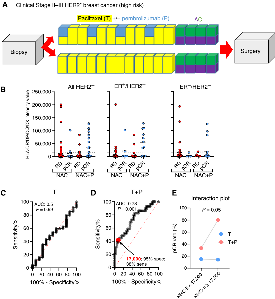
Figure 2. Tumor-specific MHC-II expression specifically predicts benefit to anti-PD-1 inhibition with NAC in high-risk HER2 - patients. A , I-SPY2 clinical trial schema depicting NAC [paclitaxel (T) in yellow, doxorubicin in purple, and cyclophosphamide in green] + pembrolizumab (P; blue) arm and NAC-only control arm. B , HLA-DR/DP/DQ/DX values by outcome for NAC-only and NAC+ pembrolizumab arms. The dotted line shows the cut-off point (17,000 units) chosen based on a calibration study comparing RPPA with a 5% tumor-specific MHC-II cut-off point. C , ROC curve for predictive capacity of tumor-specific MHC-II on pCR in NAC-alone (T) arm. D , ROC curve for predictive capacity of tumor-specific MHC-II on pCR in pembrolizumab (T+P) arm. E , Interaction plot of biomarker group (stratified at 50,000 units) and treatment arm on pCR rate. P value represents interaction term in a logistic regression model after adjusting for main effects (treatment arm and MHC-II status).
