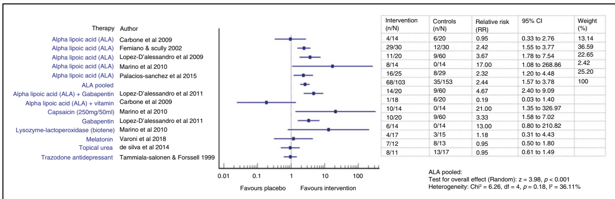
Figure 4. Forest plot showing relative risks (RRs) and 95% confidence intervals for short-term outcomes (improvement on VAS \leq 3 months) of RCTs comparing an intervention with placebo for the treatment of BMS (with pooled effect for ALA).
