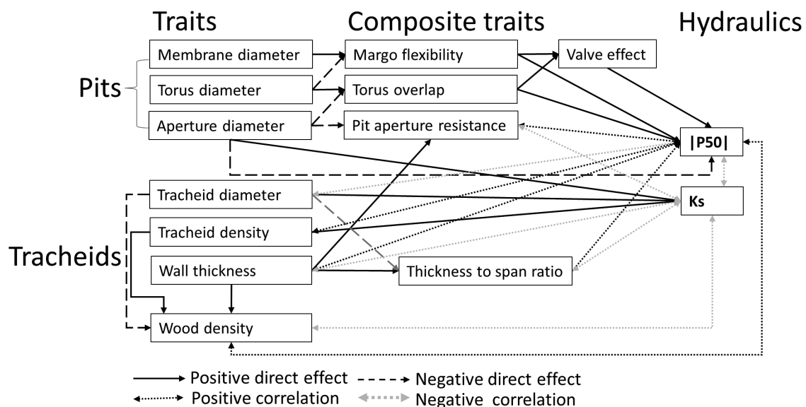
Fig. 1. A conceptual diagram visualizing our hypothesis for how pit and tracheid traits jointly determine species differences in embolism resistance (|P50|) and hydraulic conductivity ( K_s ). Our trait list is shown in Table 1.
