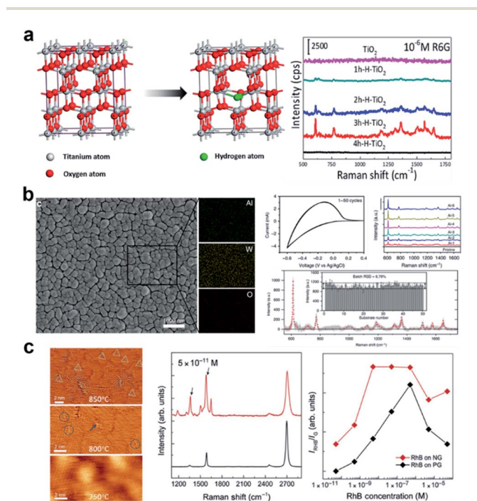
Fig. 2 Doped semiconductor substrates and SERS activity. (a) Crystal structure of TiO_2 and hydrogenated TiO_2 and Raman spectra of R6G on TiO_2 with different levels of hydrogenation. Reproduced with permission from ref. 42. Copyright 2018, American Chemical Society. (b) EDX analysis of Al-intercalated WO_3 and its SERS performance characterization. Reproduced with permission with ref. 43. Copyright 2019, Springer Nature. (c) STM images of N-doped graphene under different synthesis conditions and SERS performance characterization. Reproduced with permission from ref. 61. Copyright 2016, AAAS.
