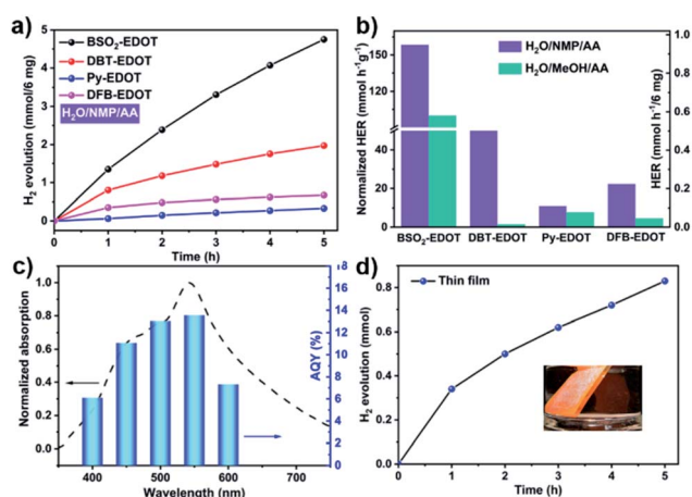
Fig. 4 (a) PHP as a function of time for 6 mg CPs under visible light irradiation. (b) Normalized HERs of CPs dispersed in AA/H 2 O/MeOH and AA/H 2 O/NMP. (c) AQYs of PHP for BSO 2 -EDOT at five different incident light wavelengths. (d) PHP from H 2 O for the BSO 2 -EDOT film (inset: film photograph) [typical conditions for PHP: 6 mg CPs dispersed in a mixed solution containing 30 ml H 2 O, 5 g SED, and 3 ml NMP under visible light irradiation at 25 °C].
