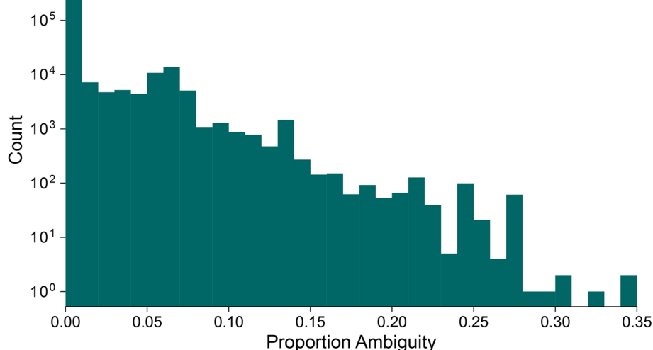
Fig. 3 Histogram of the proportion of spike protein nucleotide sites that are ambiguous (i.e. contain at least one IUPAC ambiguity code). The distribution is calculated for all SARS-CoV-2 sequences in GISAID that (i) have been designated to a Pango lineage, and (ii) have N at < 5% of sites across the whole genome, excluding UTRs
