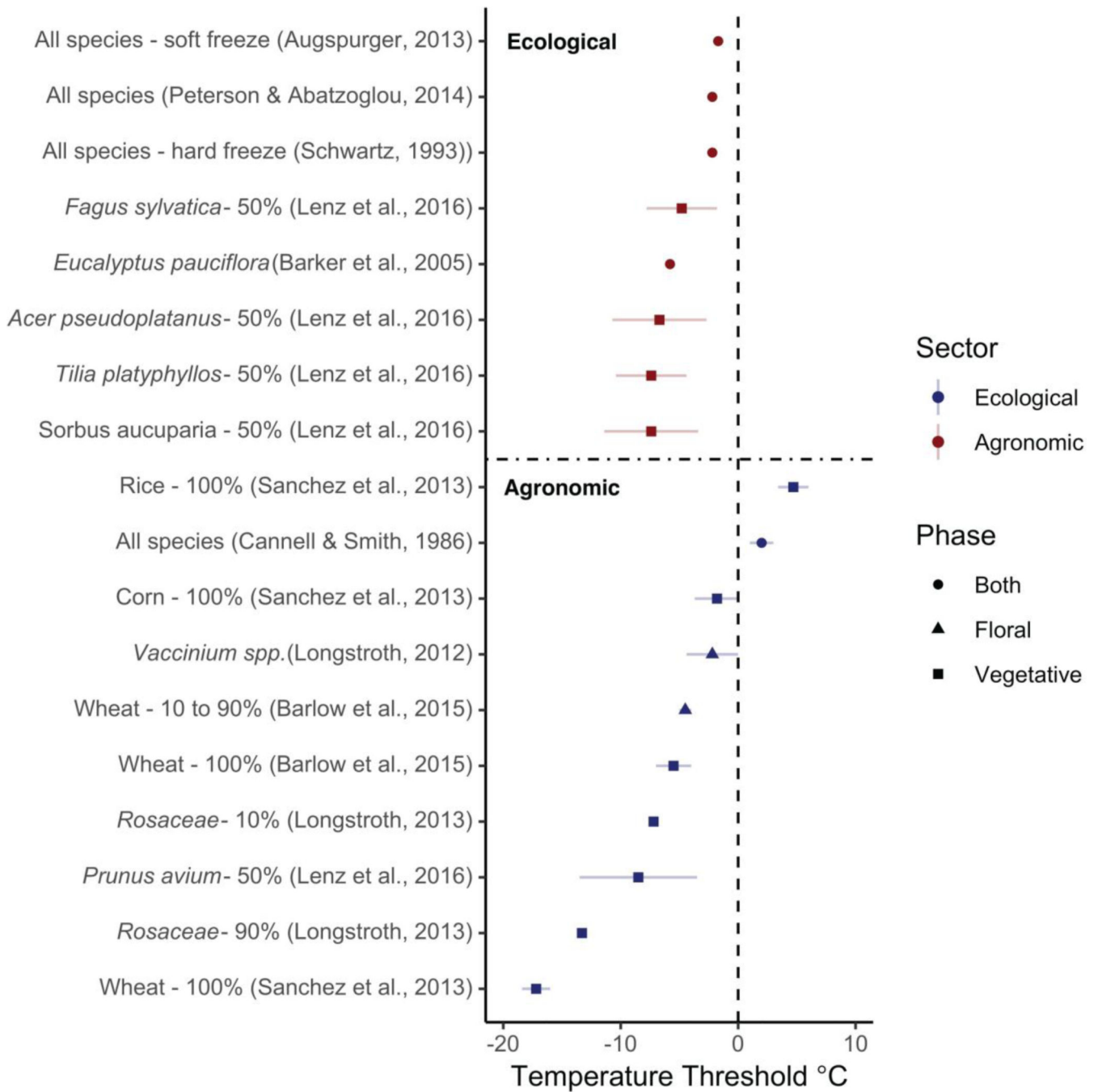
Figure 1: A comparison of damaging spring freezing temperature thresholds across ecological and agronomic studies. Each study is listed on the vertical axis along with the taxonomic group of focus. Next to the species name is the freezing definition used within that study (e.g., 100% is 100% whole plant lethality). Each point is the best estimate recorded for the temperature threshold with standard deviation if indicated in the study.
