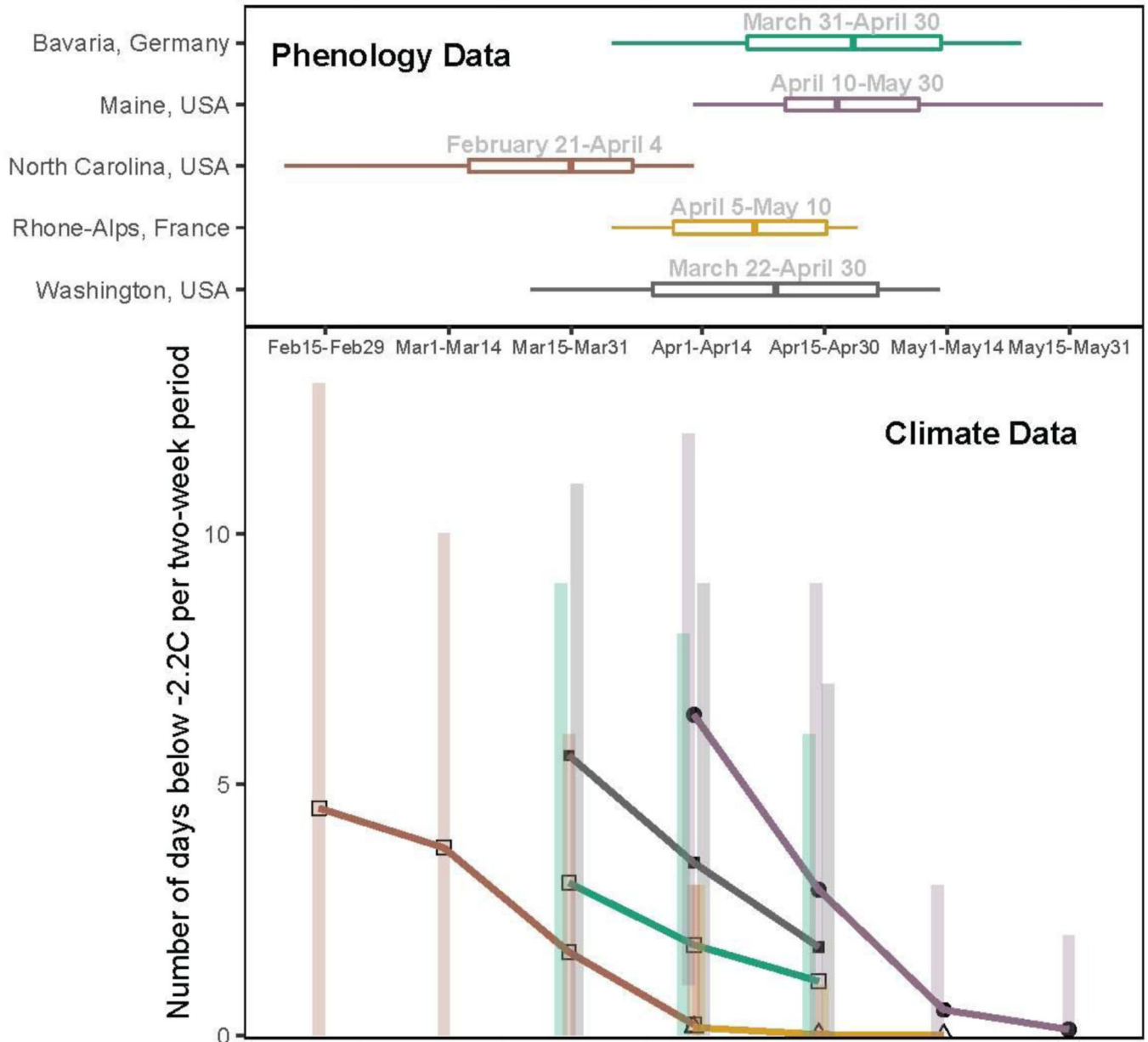
Figure 5: False spring risk can vary dramatically across regions. Here we show the period when plants are most at risk to tissue loss – between budburst and leafout (upper, lines represent the range with the thicker line representing the interquartile range) and the variation in the number of freeze days ( -2.2^{\circ}\text{C} ) (Schwartz, 1993) that occurred on average over the past 50 years for five different sites (lower, bars represent the range, points represent the mean). Data come from USA-NPN SI-x tool (1981–2016), NDVI and remote-sensing, and observational studies (1950–2016) for phenology (Schaber & Badeck, 2005; Soudani et al., 2012; USA-NPN, 2016; White et al., 2009) and NOAA Climate Data Online tool for climate (from 1950–2016). See the Supplement for further details on methods.
