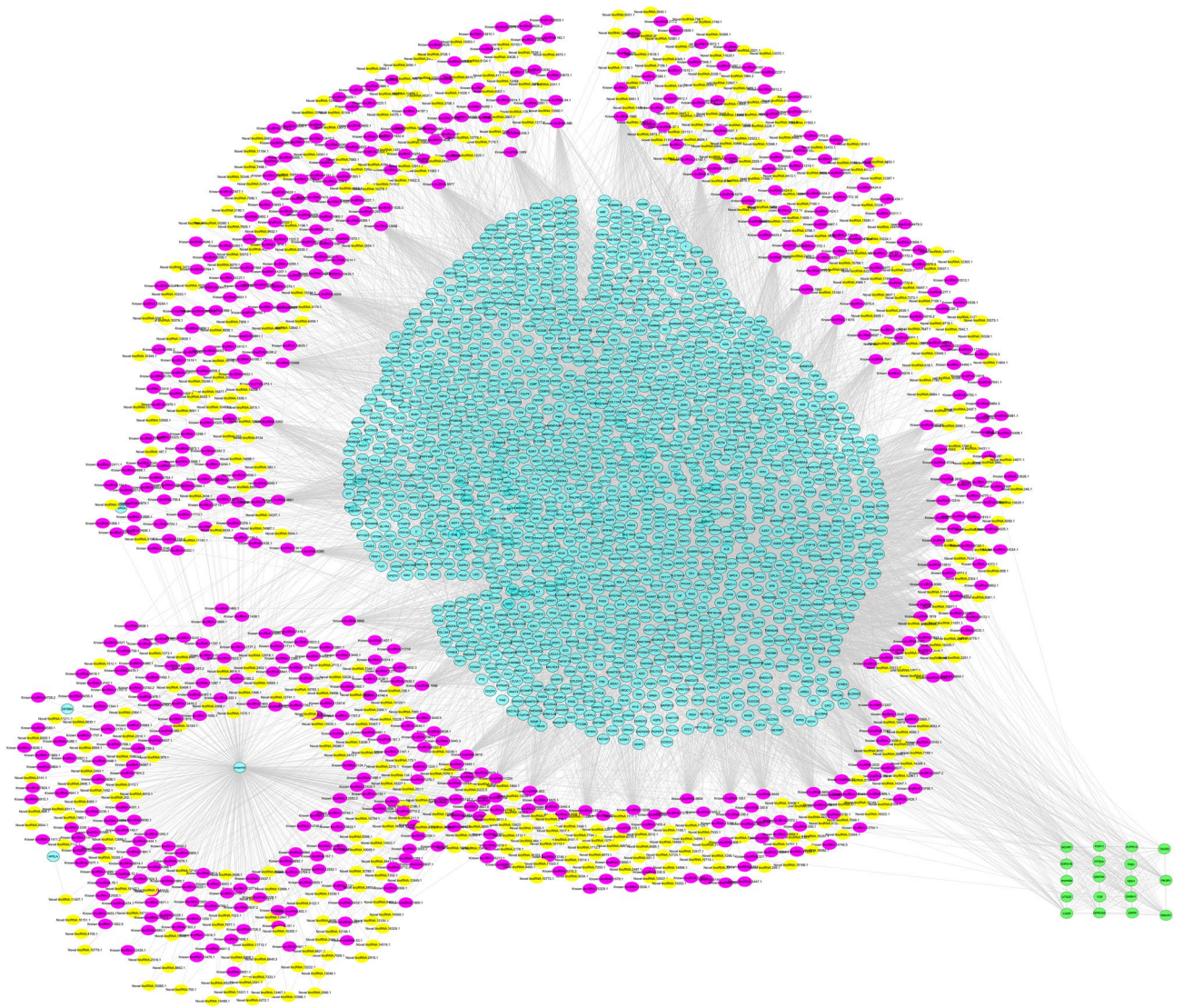
Figure 6. Final constructed network based on the known and novel lincRNAs. Purple nodes: Known lincRNAs, yellow nodes: Novel lincRNAs, Sky blue nodes: protein coding genes, green nodes: predicted module (P-value = 0.007).
