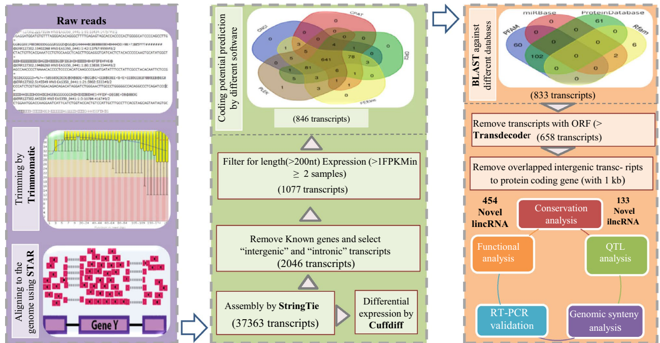
Figure 1. The bioinformatics pipeline for identifying annotated, known and novel lincRNAs. The middle and right Venn diagrams illustrate the results of the potential coding ability of the transcript using five software and blasting the transcripts against four different databases, respectively.
