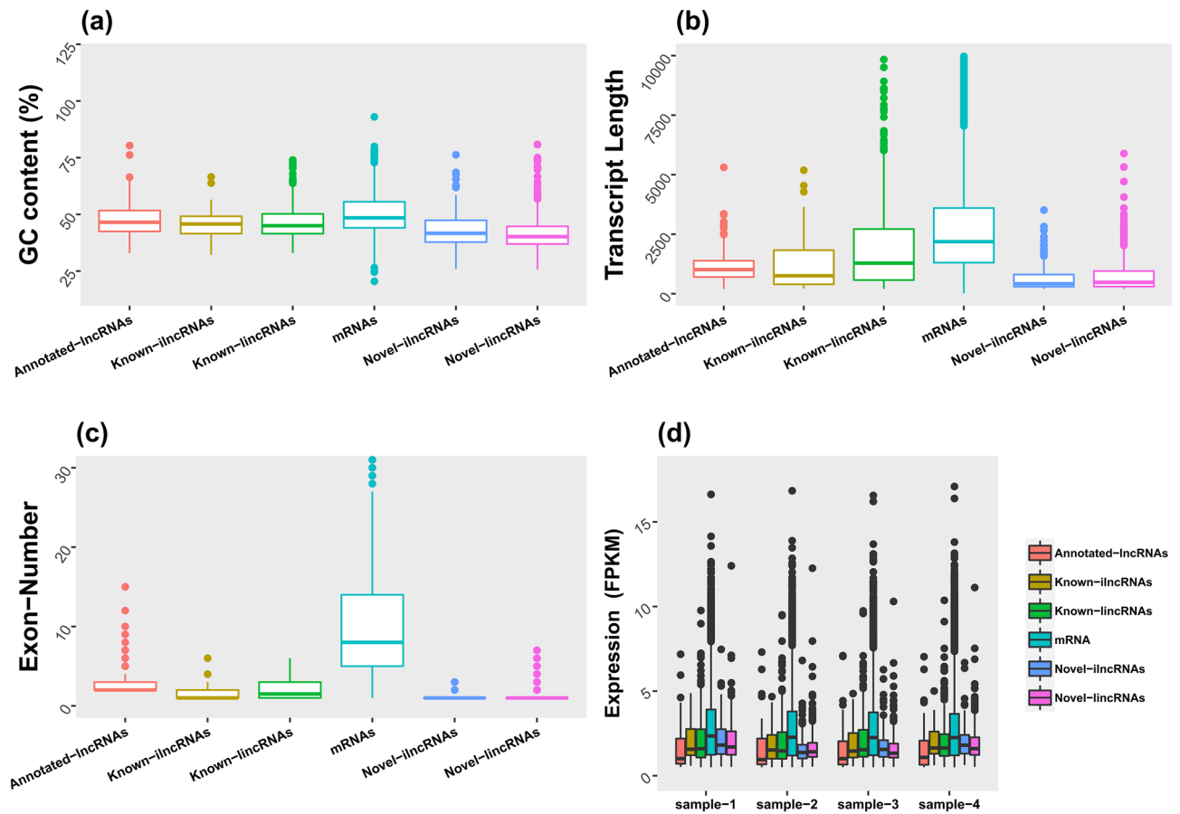
Figure 2. Comparison of (a) GC contents, (b) transcript length, (c) exon number and (d) gene expression levels of the annotated, novel and known lincRNAs with mRNAs.
