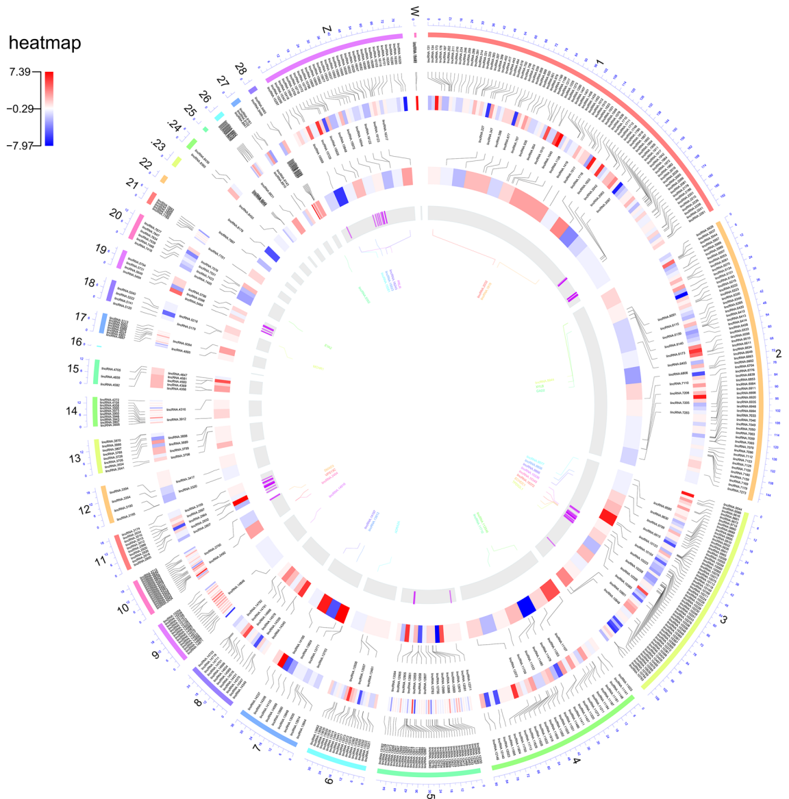
Figure 3. Circos plot represents the genome-wide distribution density of all the identified novel lincRNAs (in clockwise order). From outside to inside the plot shows the chromosomes, and the next ring the position of the novel lincRNAs, the log 2 fold change (Esfahani against Ross) of the novel lincRNAs, position of the novel lincRNAs, the log 2 fold change (Esfahani against Ross) of the novel lincRNAs, the location of Residual feed intake QTLs from animal QTL database and the names of promising lincRNAs and mRNAs pairs associate with Residual feed intake. Red heatmap colors represent the higher expression of the gene in Esfahani than Ross breed.
