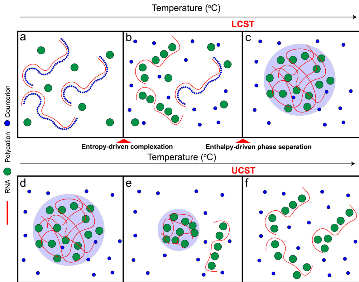
Figure 5. The interplay between entropy-driven complexation and enthalpy-driven phase separation may underlie the closed-loop phase behavior of RNA-polycation mixtures. A scheme summarizing the proposed mechanism for the closed-loop phase diagram exhibited by RNA-polycation mixtures. Panels (a-f) are the complexation and phase separation behavior of the system with increasing temperatures. RNA is drawn as red chains, counter-ions are drawn as blue circles, and polycations are drawn as green circles.
