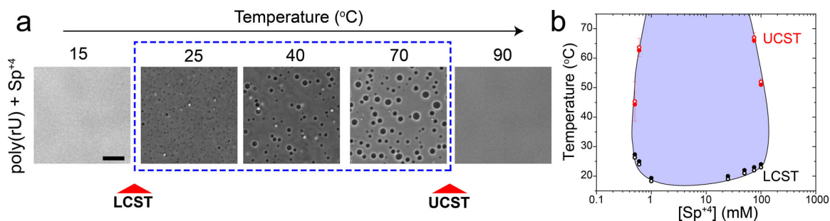
Figure 2. RNA-spermine mixtures have coexisting LCST and UCST phase transitions.
