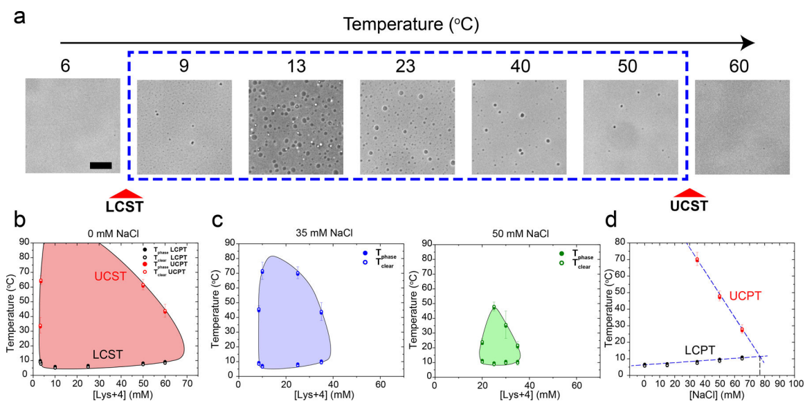
Figure 3. The closed-loop phase behavior of RNA-polycation mixtures is sensitive to the ionic strength of the buffer.
