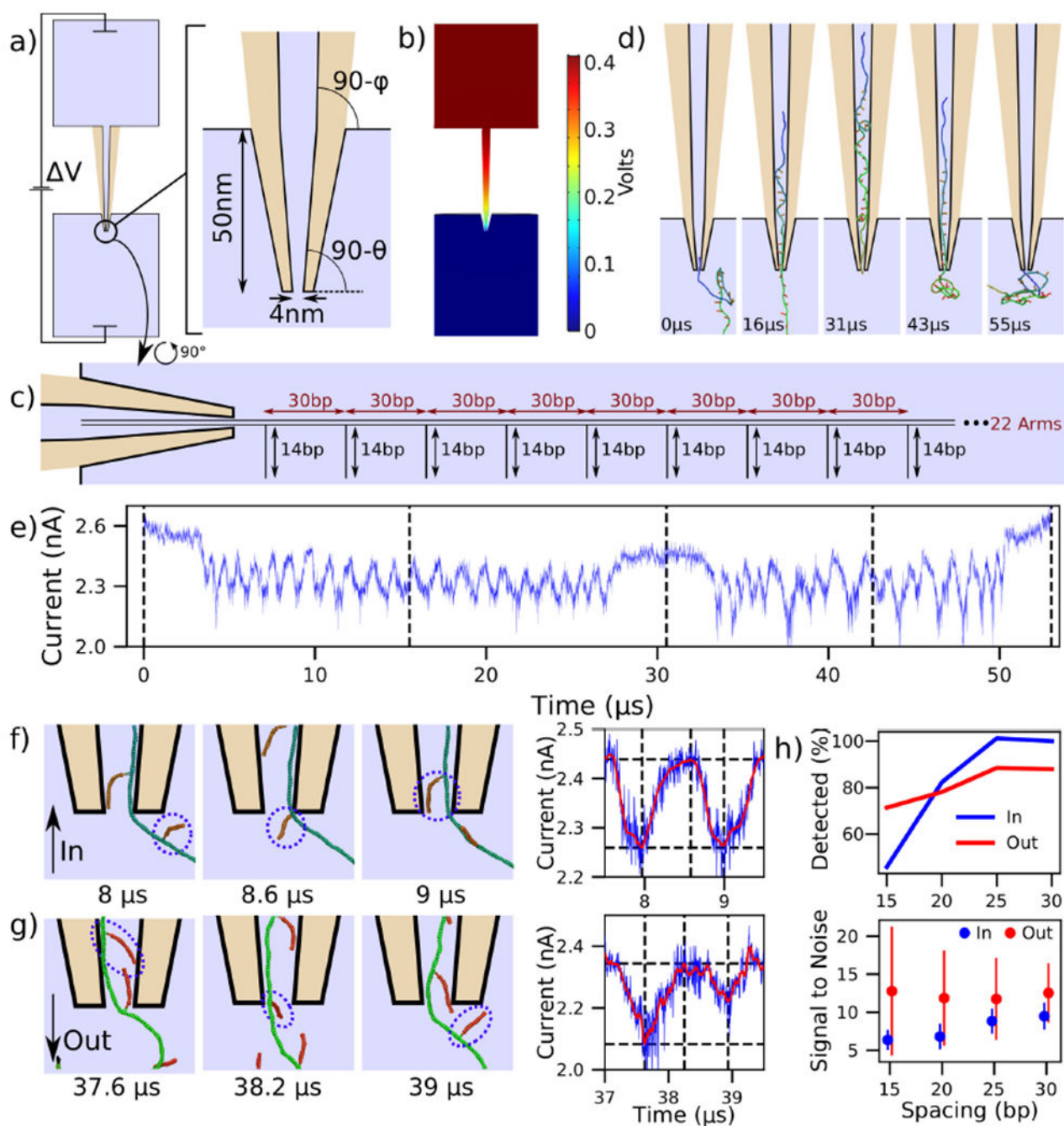
Figure 4: Modeling DNA data storage readout. (a) Schematic of a capillary used in DNA storage experiments [6, 37] and the zoomed-in view of the tip geometry. The angles \theta and \phi are 4.9 and 1.2 degrees, respectively. Light blue colored areas represent the simulation volume whereas the tan color represents the glass capillary. (b) Distribution of the electrostatic potential corresponding to a 400 mV bias applied to pull a DNA construct into the capillary. (c) Schematic of the DNA data storage construct entering the capillary. (d) Sequence of snapshots illustrating a simulation of the construct's translocation into and out of the
