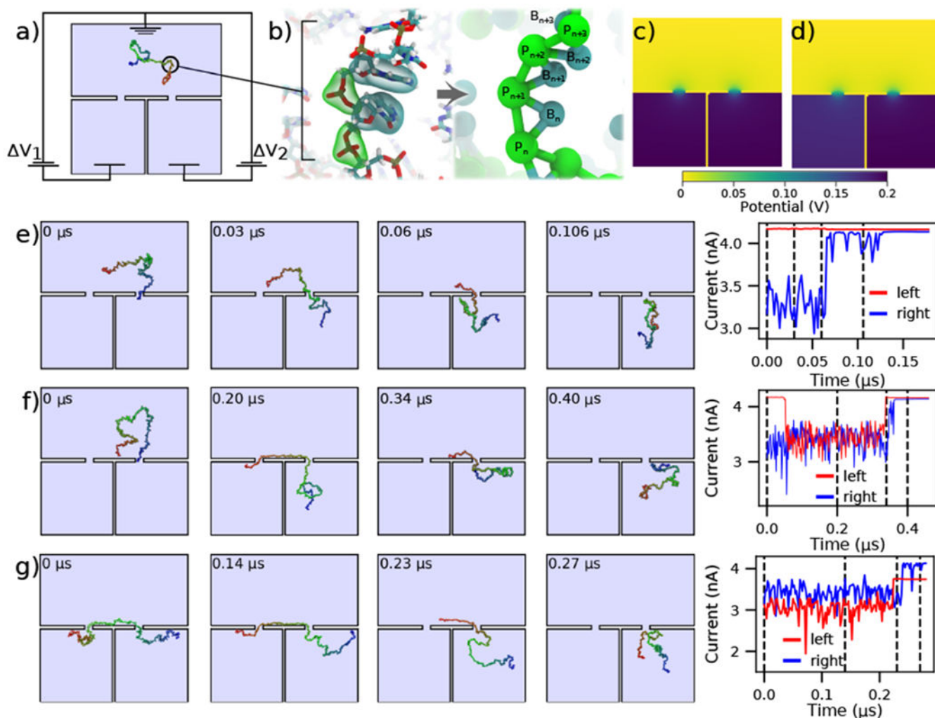
Figure 3: Modeling capture and translocation of ssDNA in a double nanopore system. (a) A previously described double nanopore system [43], consisting of two identical pores of 1 nm radius and length, separated by 15 nm. The nanopores lead to separate volumes which are separated by a 1 nm thick wall. Here, we consider a situation where the voltage bias \Delta V_1 and \Delta V_2 in each of the bottom chambers can be independently controlled relative to the top compartment, which is grounded. A 150 nucleotide ssDNA molecule is modeled at two-beads-per-nucleotide resolution. (b) Schematic of the two-beads-per-nucleotide model of ssDNA, adapted from an earlier work [48]. Each nucleotide is represented by a backbone bead P and a base bead B . (c,d) Distribution of the electrostatic potential under conditions of translocation arrest, \Delta V_1 = \Delta V_2 = 200 mV (panel c), and directed translocation, \Delta V_1 = 180 mV and \Delta V_2 = 200 mV (panel d). (e,f) Single (panel e) and double (panel f) nanopore capture of ssDNA. The simulations begin with one end of the DNA strand captured in the right nanopore. The voltage drop across both pores is 200 mV (panel c). The right panel shows the ionic current through the left and right nanopores for the corresponding simulation trajectory. (g) Directional transport of ssDNA through the double nanopore system. The simulation begins having two ends of ssDNA symmetrically threaded into the
