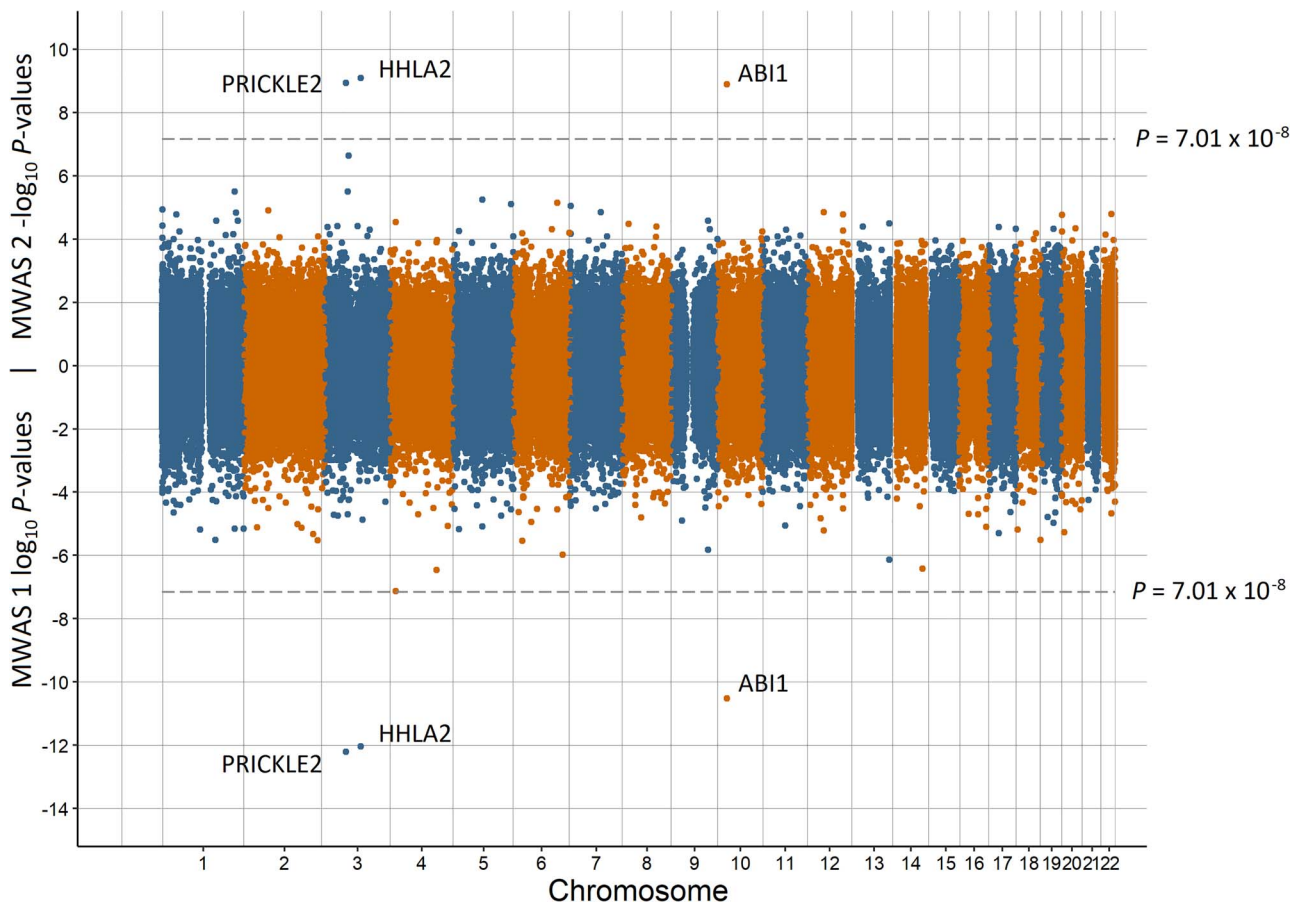
Figure 1. Miami plot of the observed P-values of each CpG site for an association with preterm birth. \log_{10} P-values are shown for MWAS 1 and -\log_{10} P-values are shown for MWAS 2. The dotted lines indicate methylome-wide significance ( P = 7.01 \times 10^{-8} ). The annotation of genes for significant sites is reported by missMethyl for MWAS 1 and by OSCA for MWAS 2.
