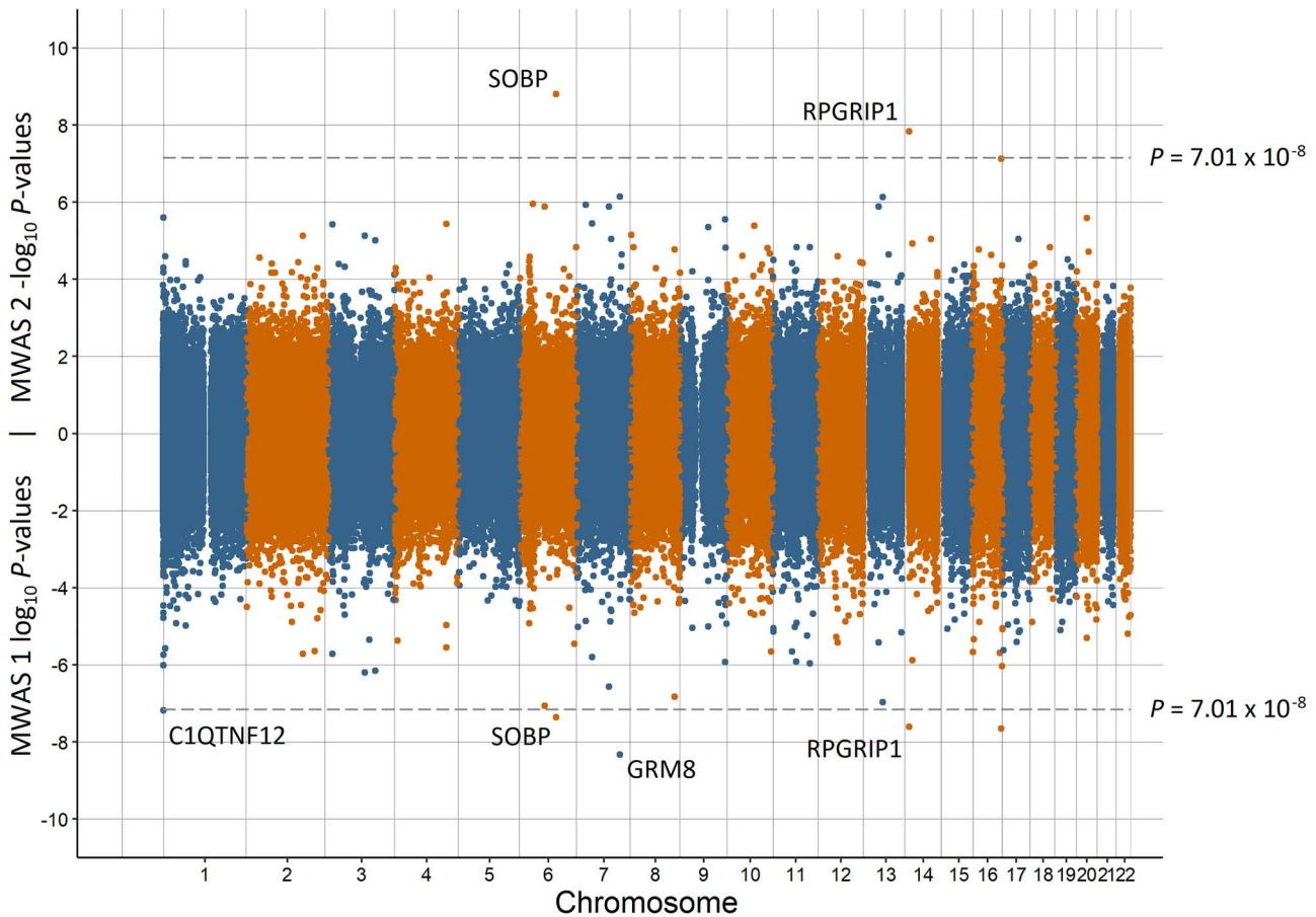
Figure 2. Miami plot of the observed P-values of each CpG site for an association with low birth weight. \log_{10} P-values are shown for MWAS 1 and -\log_{10} P-values are shown for MWAS 2. The dotted lines indicate methylome-wide significance ( P = 7.01 \times 10^{-8} ). The annotation of genes for significant sites is reported by missMethyl for MWAS 1 and by OSCA for MWAS 2.
