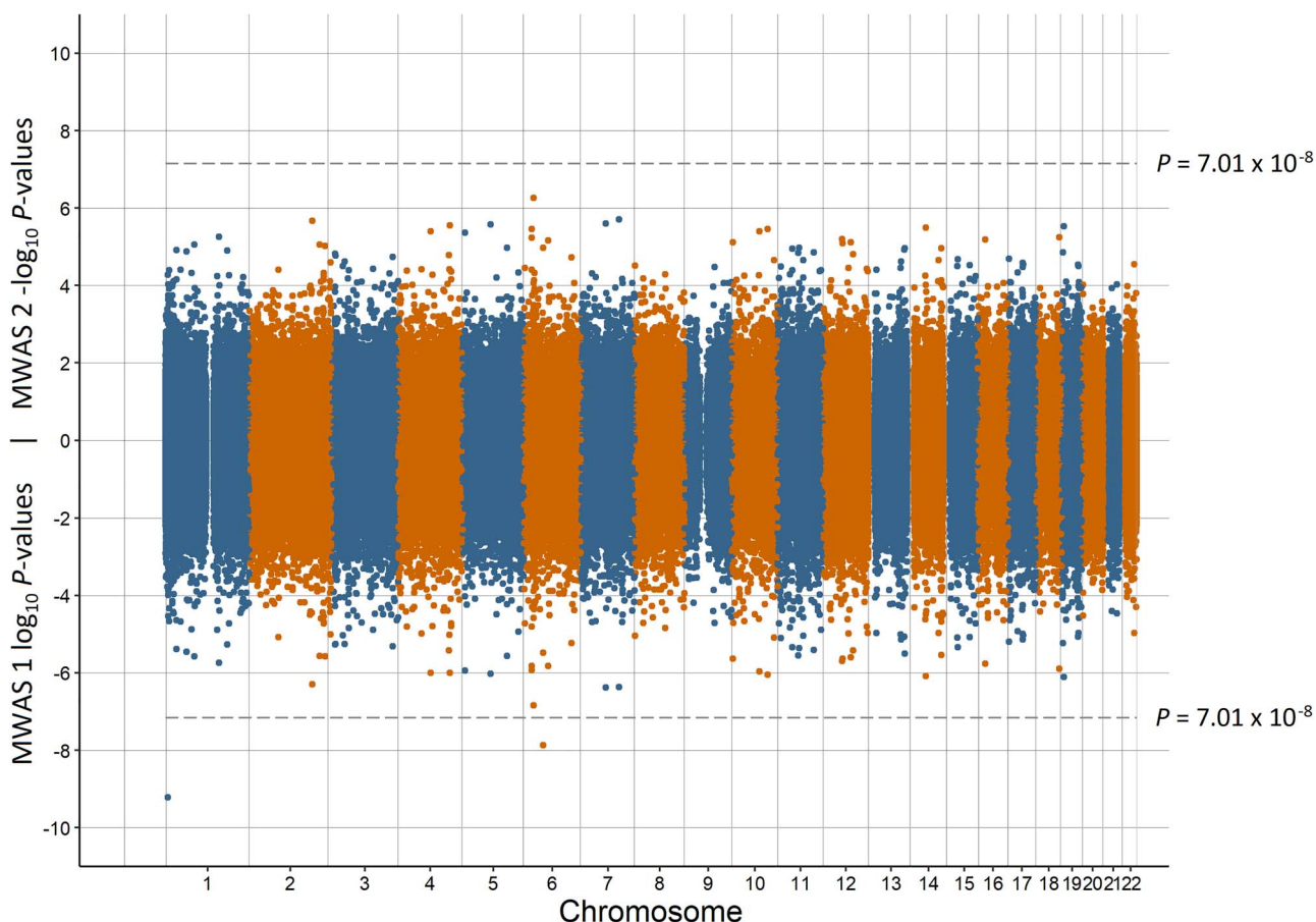
Figure 5. Miami plot of the observed P -values of each CpG site for an association with MDD. \log_{10} P -values are shown for MWAS 1 and -\log_{10} P -values are shown for MWAS 2. The dotted lines indicate methylome-wide significance ( P = 7.01 \times 10^{-8} ). Significant sites did not annotate to any genes.
