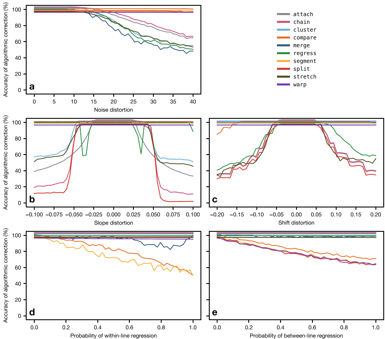
Fig. 4 Mean accuracy of the ten algorithms in response to the five eye-tracking phenomena. For example, some algorithms ( attach , chain , cluster , merge , regress , and stretch ) are adversely affected as the noise level is increased, while the other algorithms are
