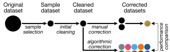
Fig. 6 Pipeline for testing the algorithms on a natural dataset. The original dataset was first reduced to a smaller sample, which then underwent some initial cleaning steps. This cleaned dataset was then corrected by the ten algorithms and two human correctors, whose corrections were merged to form the gold standard. Performance is measured by how closely the algorithmic corrections match the gold standard correction
