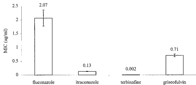
FIG. 1. Mean MICs of fluconazole, itraconazole, terbinafine, and griseofulvin for 217 dermatophytes by the proposed method for in vitro susceptibility testing.
