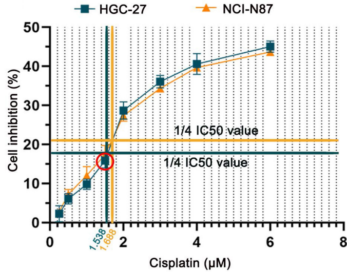
SUPPLEMENTARY FIG. 1. The cell inhibition of NCI-N87 cells and HGC-27 cells in the control group treated with various concentrations (0, 0.25, 0.5, 1, 1.5, 2, 3, 4, and 6 \mu\text{M} ) of cisplatin for 48 hours. To investigate whether knockdown of SGK1 could promote the cisplatin sensitivity, a low-dose cisplatin (1.5 \mu\text{M} , a quarter of the IC50 of the control cells) was chosen for the subsequent experiments.
