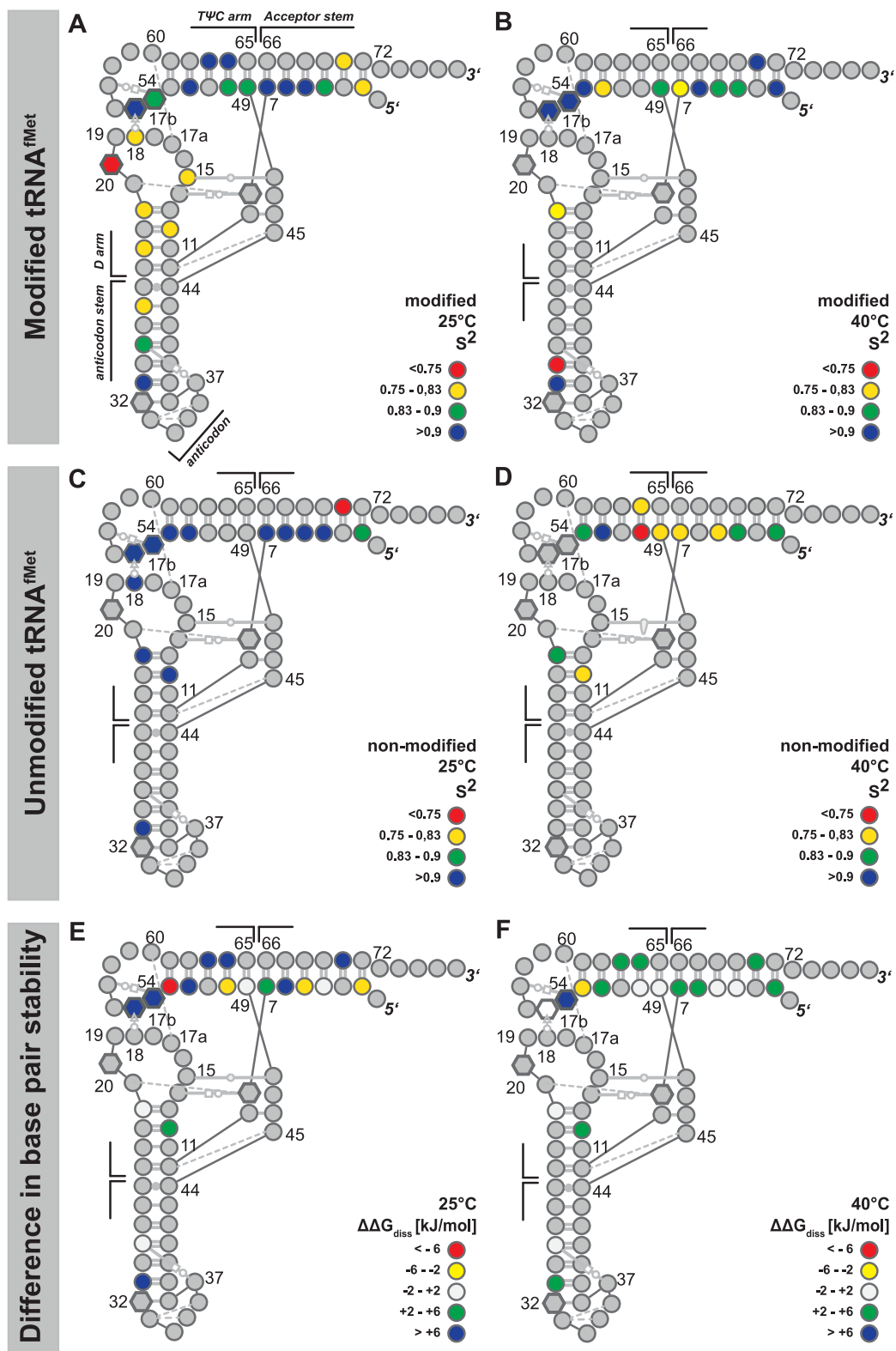
Figure 6. Comparison of local dynamics and base pair stabilities for modified and unmodified tRNA fMet . Nucleotide-resolved representation of the L-shaped structure that is color coded to represent the S 2 order parameter for (A) native tRNA at 25°C and (B) at 40°C; (C) unmodified tRNA at 25°C and (D) at 40°C. The base interactions are annotated according to the nomenclature of Leontis and Westhof (112), modified residues are represented by hexagons instead of circles. The differences in the stabilities of corresponding base pairs ( \Delta\Delta G_{diss} = \Delta G_{diss}^{modified} - \Delta G_{diss}^{non-modified} ) are given for (E) 25°C and (F) 40°C. Positive values shown in blue and green mean that modified tRNA is more stable than unmodified tRNA. In contrast, negative \Delta\Delta G_{diss} values shown in yellow and red show that unmodified tRNA is more stable than modified tRNA. White highlighted nucleotides represent only a minor difference in \Delta\Delta G_{diss} between both tRNAs. All data is summarized in Supplementary Tables S9-S12 and S15-S16.
