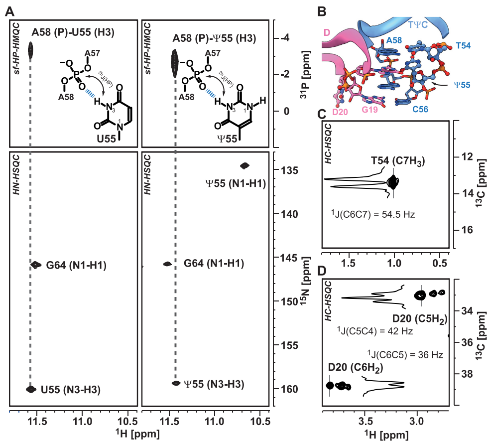
Figure 4. NMR spectroscopic signatures of modified residues. (A) Characterization of N3H3-phosphate group hydrogen bonds through sofast- ^1\text{H} , ^{31}\text{P} HMQC experiments. The H3 atom of residues U55 (left panel) and \Psi 55 (right panel) with the phosphate group of residues A58 is correlated and related to the according HN cross peaks of the corresponding ^1\text{H} , ^{15}\text{N} HSQC, which are given in the panels below. (B) Placement of modified residues within the core region, which are establishing the interaction between D- (pink) and T \Psi C-loop (blue) as mapped by crystal structure (PDB: 3CW6). (C) The C7H 3 cross peak of T54 detected in ^1\text{H} , ^{13}\text{C} HSQC and (D) the methylene-group cross peaks of D20 C5H 2 and C6H 2 in ^1\text{H} , ^{13}\text{C} HSQC. The inserts in (C) and (D) reflect the traces along the ^{13}\text{C} -dimension to highlight the multiplet structure and reveal the respective ^1J_{\text{CC}} couplings. Experimental details are provided in an extended figure caption in SI.
