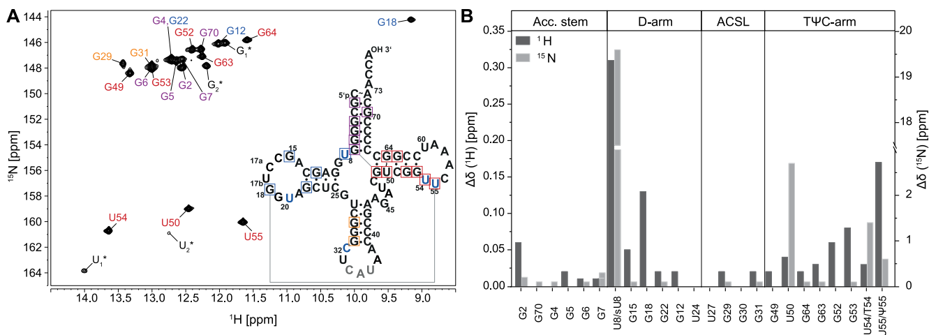
Figure 3. 2D- ^1\text{H} , ^{15}\text{N} -BEST-TROSY experiment of unmodified tRNA Met with secondary structure (A) and analysis of chemical shift differences between modified and non-modified tRNA (B). (A) The BEST-TROSY spectrum of the non-modified tRNA Met was acquired at 25°C. The secondary structure of the non-modified tRNA Met is shown. Unambiguously assigned imino peaks are highlighted in either purple (acceptor stem), blue (D-arm), orange (ACSL) or red (T \Psi C-arm). (B) Chemical shift difference between the imino resonances of the non-modified and modified tRNA Met construct was calculated as absolute values of the difference between corresponding imino signals (Supplementary Table S1 and Supplementary Table S2). Experimental details are provided in an extended figure caption in SI.
