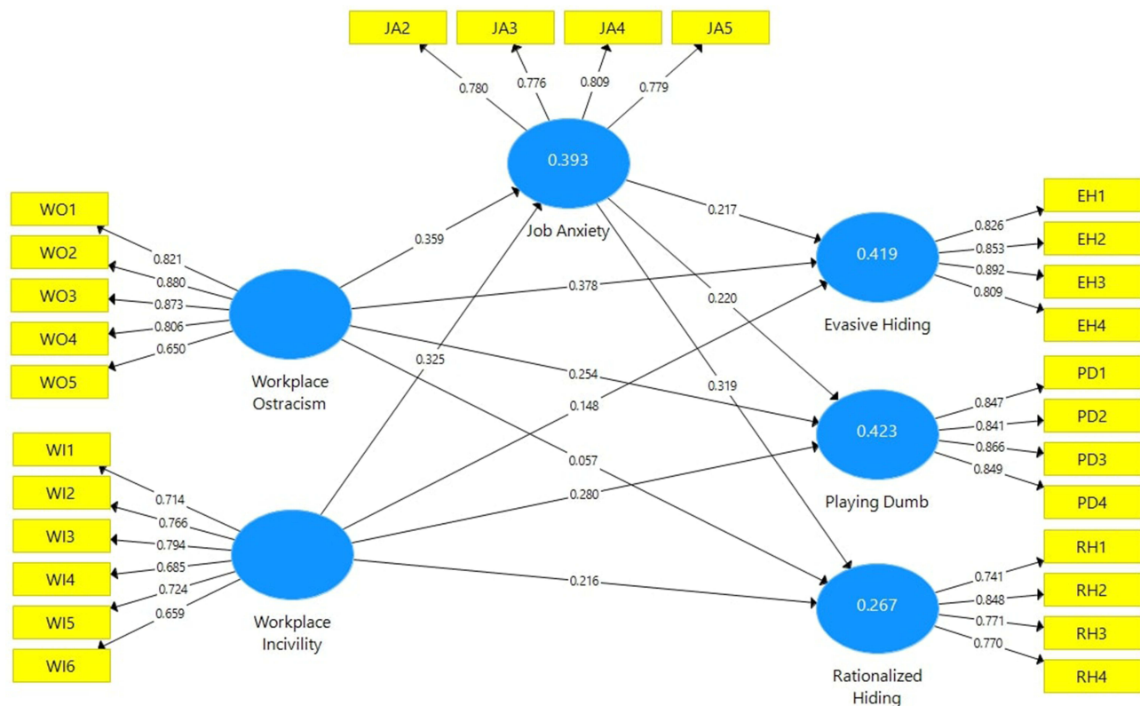
Figure 2 Measurement Model.
