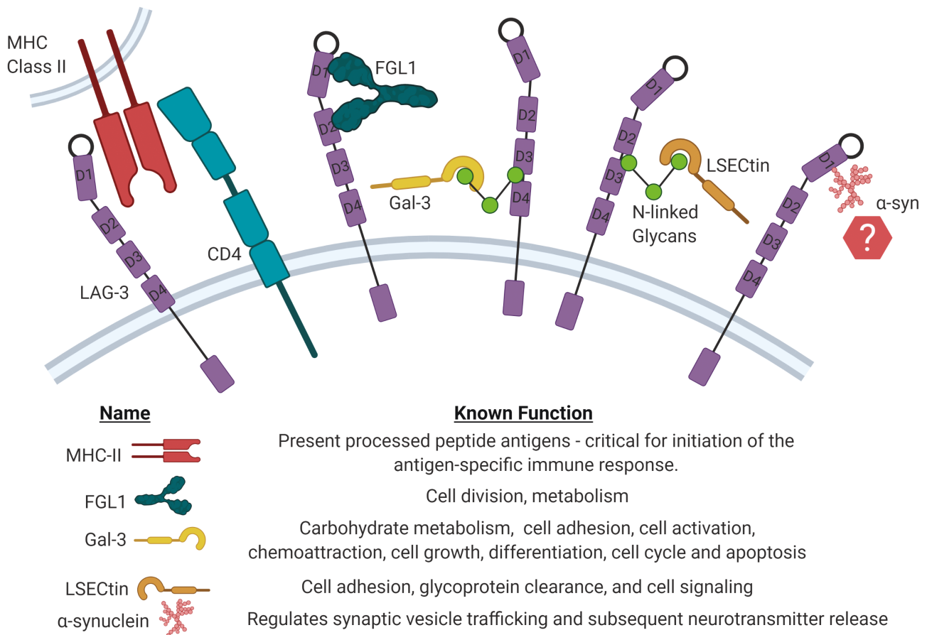
Figure 1. Possible LAG-3 ligands and their functions; MHC-II, FGL1, Gal-3, LSEctin, and \alpha -synuclein. The interaction between LAG-3 and MHC-II is believed to occur between the D1 loop of LAG-3 binding to a membrane-proximal site on MHC-II, similar to the defined MHC-II/CD4 binding site which is shown here for reference. FGL1 binds to LAG-3 at two sites in D1 and D2, while Gal-3 and LSEctin bind to N-linked glycans at glycosylation sites and \alpha -syn has been shown to bind to the D1 domain of LAG-3.
