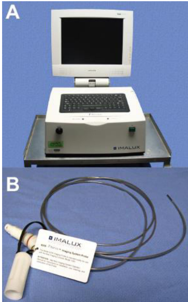
Figure 1. A) Imalux Niris OCT Imaging System. B) 2.7mm diameter by 5M length flexible probe.
