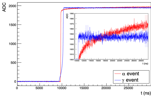
Fig. 1 Baseline-removed and pole-zero corrected waveforms from PONAma-1 events, taken with the TUBE scanning system. Both the bulk \gamma event (in blue) and the surface \alpha event, taken with the source incident at r = -7.5 mm (in red), have 2615 keV of energy. The waveform regions used to calculate the DCR parameter for each waveform, determined as described in Sect. 2.4, are indicated by the shaded boxes, shown in the same color as the waveform they correspond to
